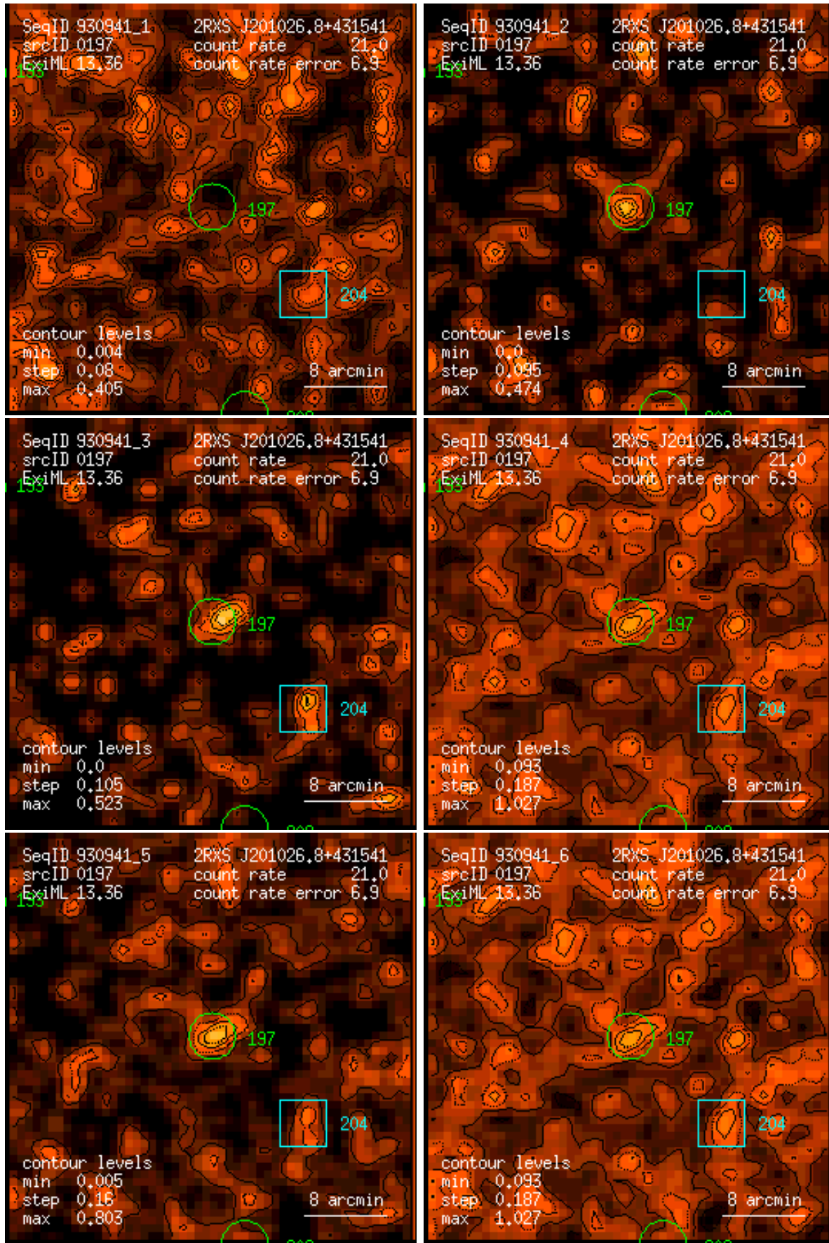
Figure 197: RASS 930941: detection 0197: band rate images, Gaussian filter: (1) PSPC channels 11 – 41, (2) 52 – 90, (3) 91 – 201, (4) 11 – 235, (5) 52 – 201, (6) 11 – 201. Broad band rates in counts/ks. Band rate contour levels in counts/ks/arcmin 2 .
