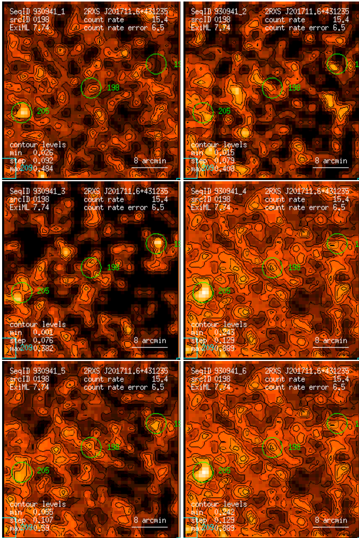
Figure 198: RASS 930941: detection 0198: band rate images, Gaussian filter: (1) PSPC channels 11 – 41, (2) 52 – 90, (3) 91 – 201, (4) 11 – 235, (5) 52 – 201, (6) 11 – 201. Broad band rates in counts/ks. Band rate contour levels in counts/ks/arcmin 2 .
