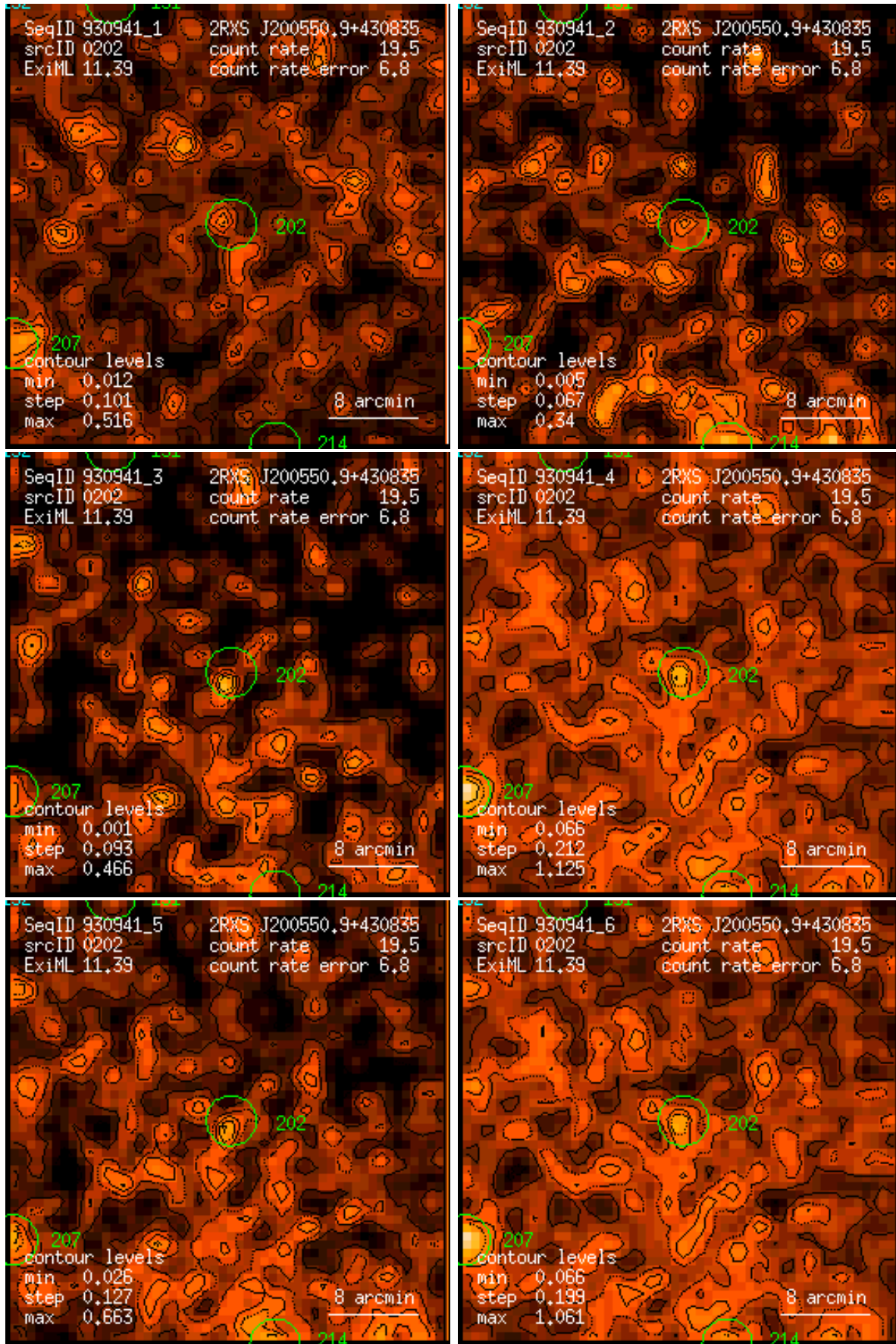
Figure 202: RASS 930941: detection 0202: band rate images, Gaussian filter: (1) PSPC channels 11 – 41, (2) 52 – 90, (3) 91 – 201, (4) 11 – 235, (5) 52 – 201, (6) 11 – 201. Broad band rates in counts/ks. Band rate contour levels in counts/ks/arcmin 2 .
