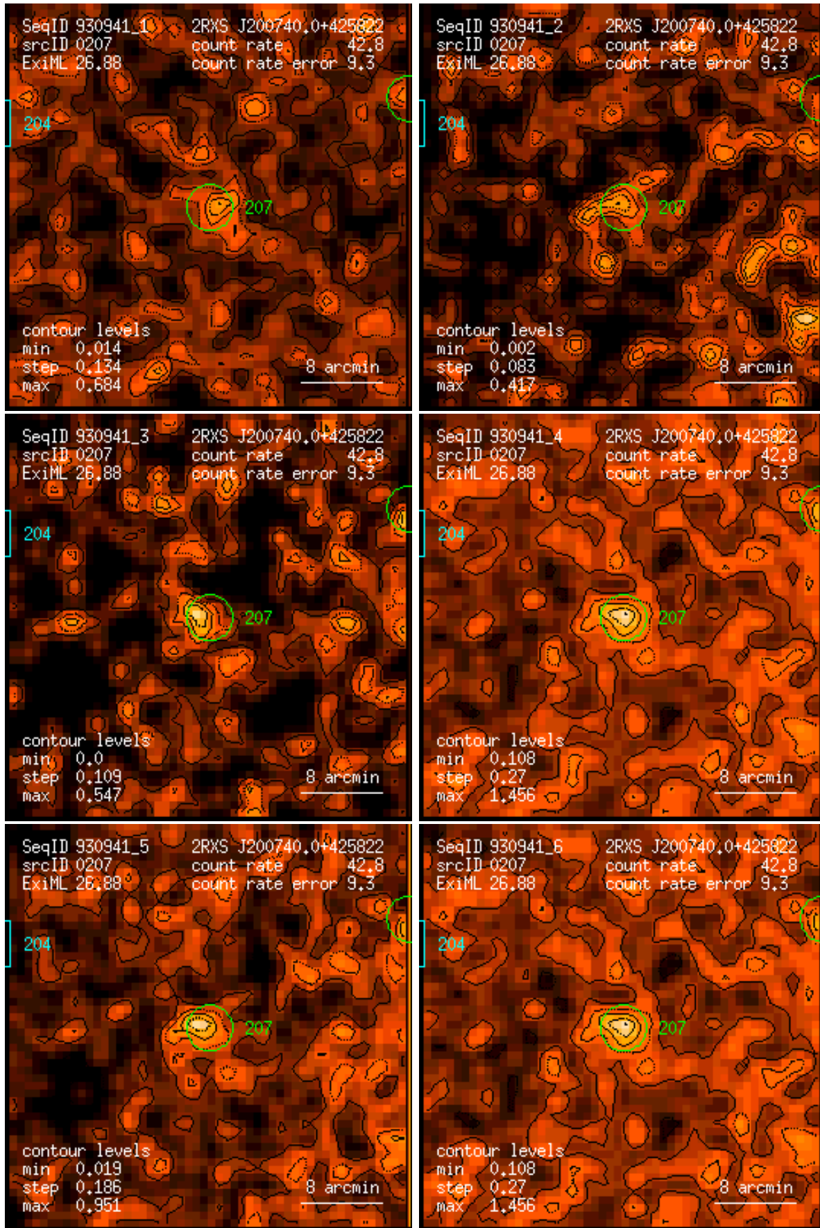
Figure 207: RASS 930941: detection 0207: band rate images, Gaussian filter: (1) PSPC channels 11 – 41, (2) 52 – 90, (3) 91 – 201, (4) 11 – 235, (5) 52 – 201, (6) 11 – 201. Broad band rates in counts/ks. Band rate contour levels in counts/ks/arcmin 2 .
