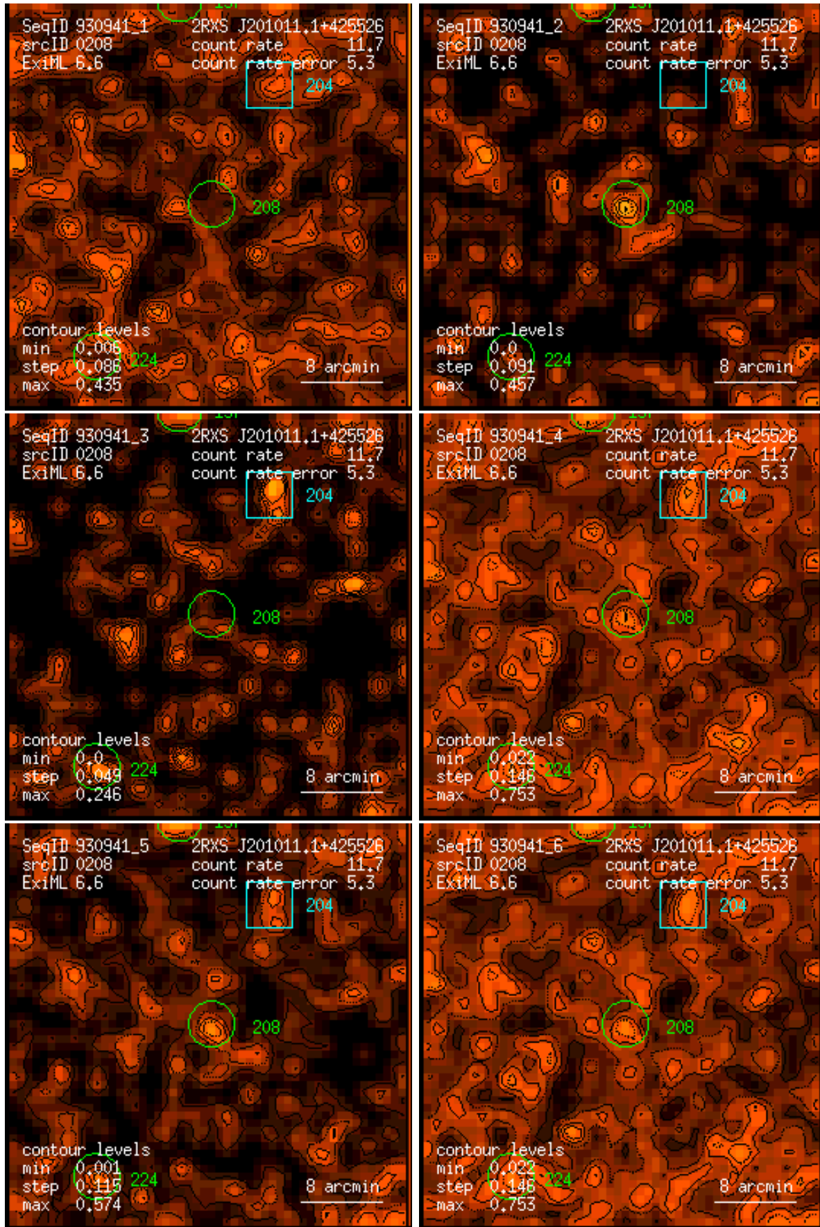
Figure 208: RASS 930941: detection 0208: band rate images, Gaussian filter: (1) PSPC channels 11 – 41, (2) 52 – 90, (3) 91 – 201, (4) 11 – 235, (5) 52 – 201, (6) 11 – 201. Broad band rates in counts/ks. Band rate contour levels in counts/ks/arcmin 2 .
