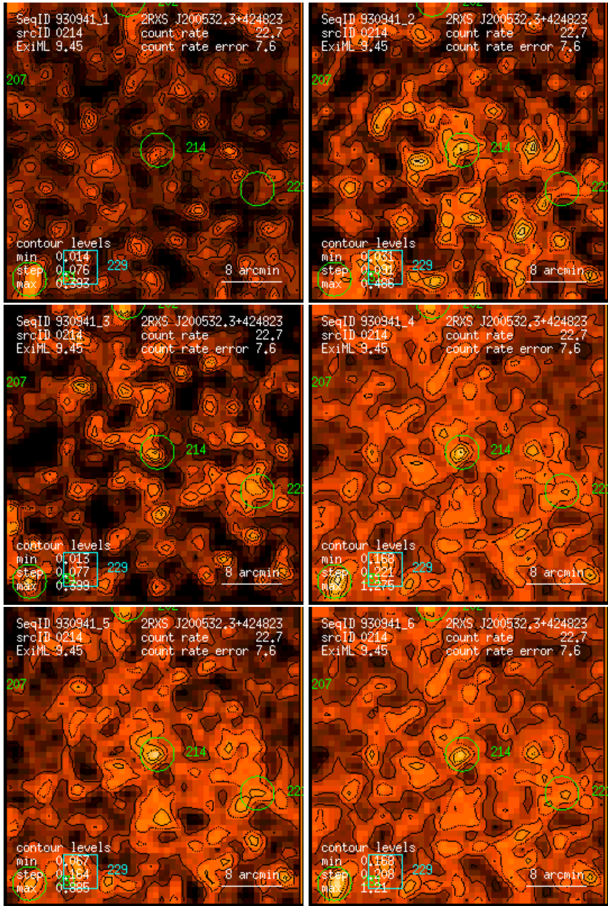
Figure 214: RASS 930941: detection 0214: band rate images, Gaussian filter: (1) PSPC channels 11 – 41, (2) 52 – 90, (3) 91 – 201, (4) 11 – 235, (5) 52 – 201, (6) 11 – 201. Broad band rates in counts/ks. Band rate contour levels in counts/ks/arcmin 2 .
