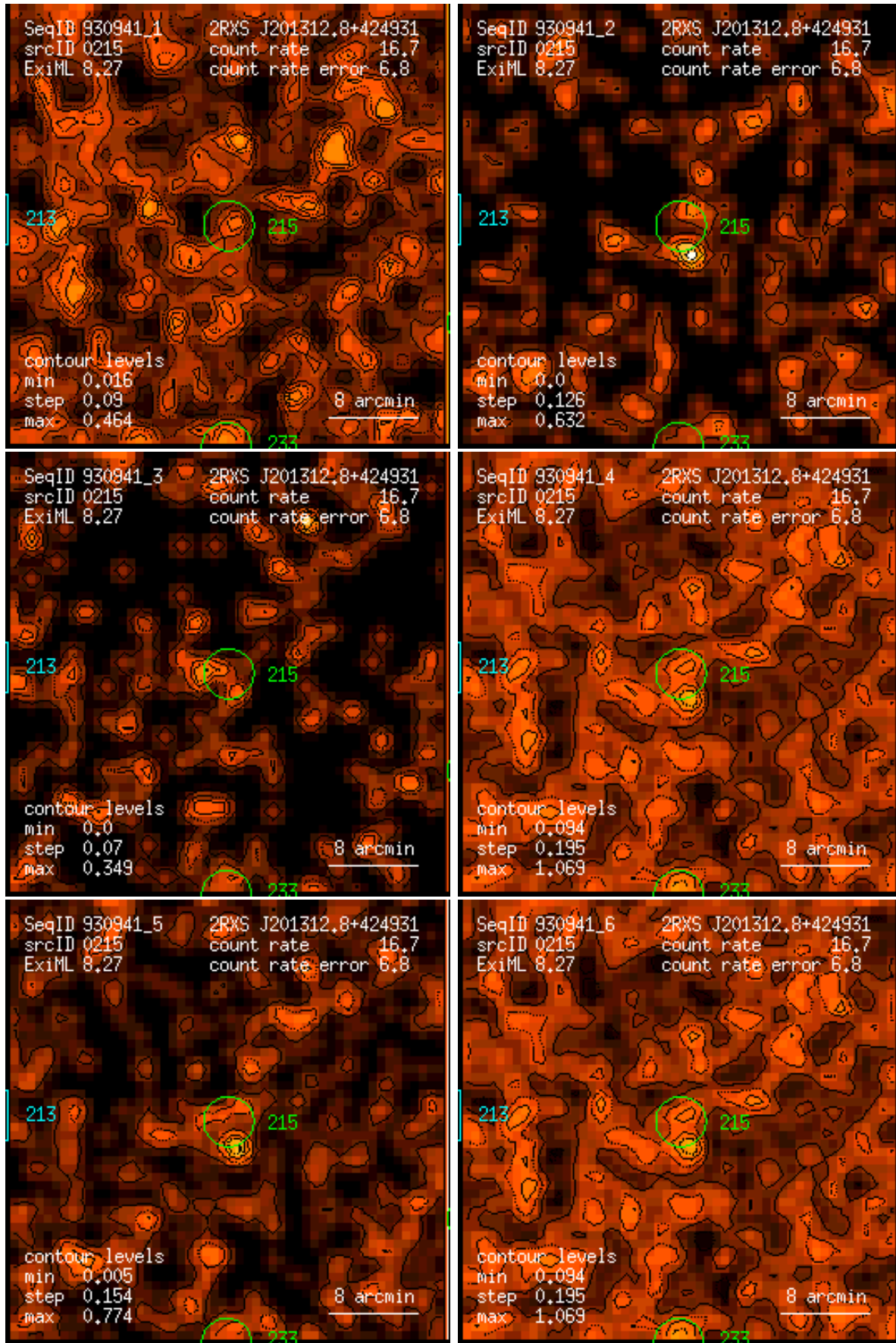
Figure 215: RASS 930941: detection 0215: band rate images, Gaussian filter: (1) PSPC channels 11 – 41, (2) 52 – 90, (3) 91 – 201, (4) 11 – 235, (5) 52 – 201, (6) 11 – 201. Broad band rates in counts/ks. Band rate contour levels in counts/ks/arcmin 2 .
