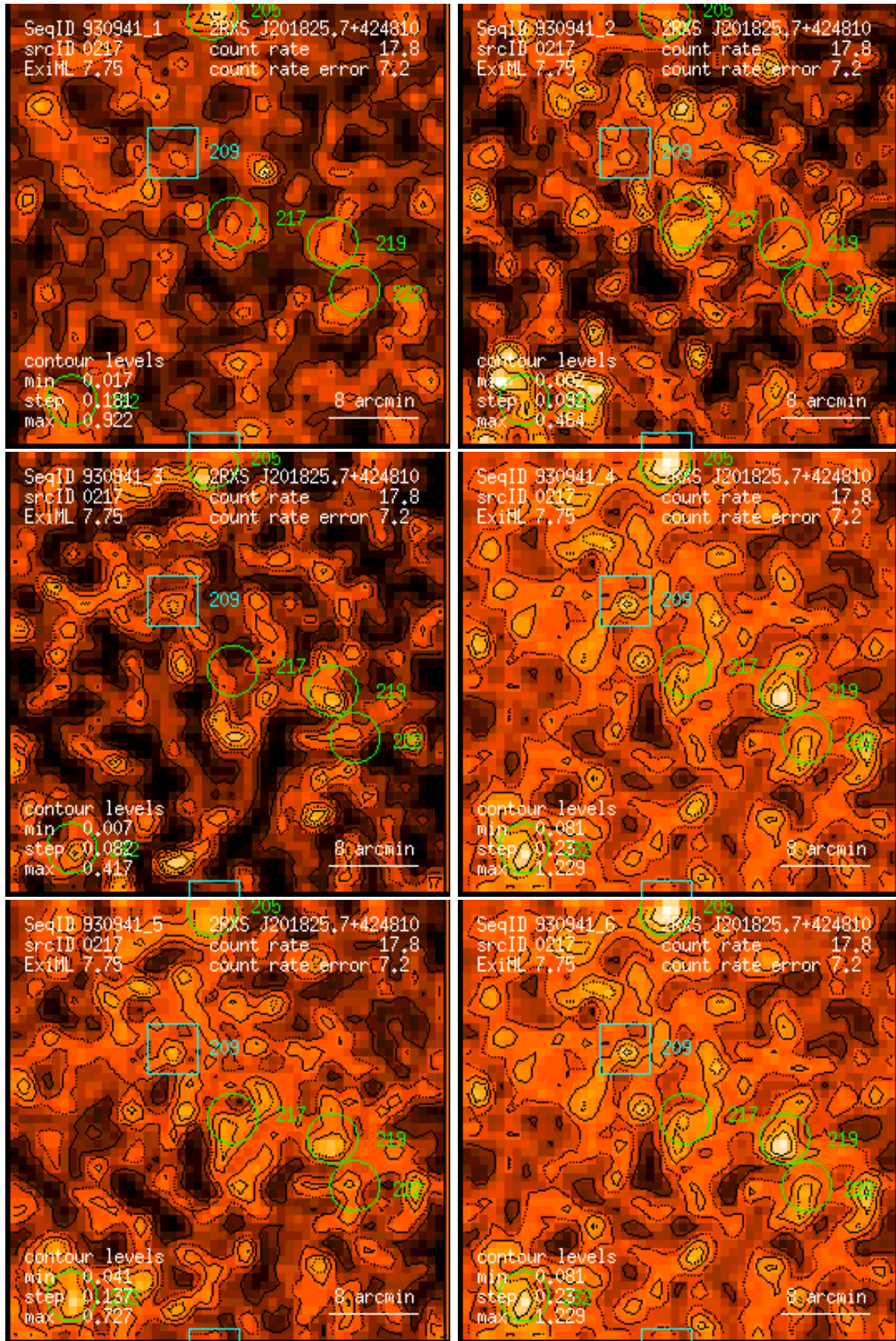
Figure 217: RASS 930941: detection 0217: band rate images, Gaussian filter: (1) PSPC channels 11 – 41, (2) 52 – 90, (3) 91 – 201, (4) 11 – 235, (5) 52 – 201, (6) 11 – 201. Broad band rates in counts/ks. Band rate contour levels in counts/ks/arcmin 2 .
