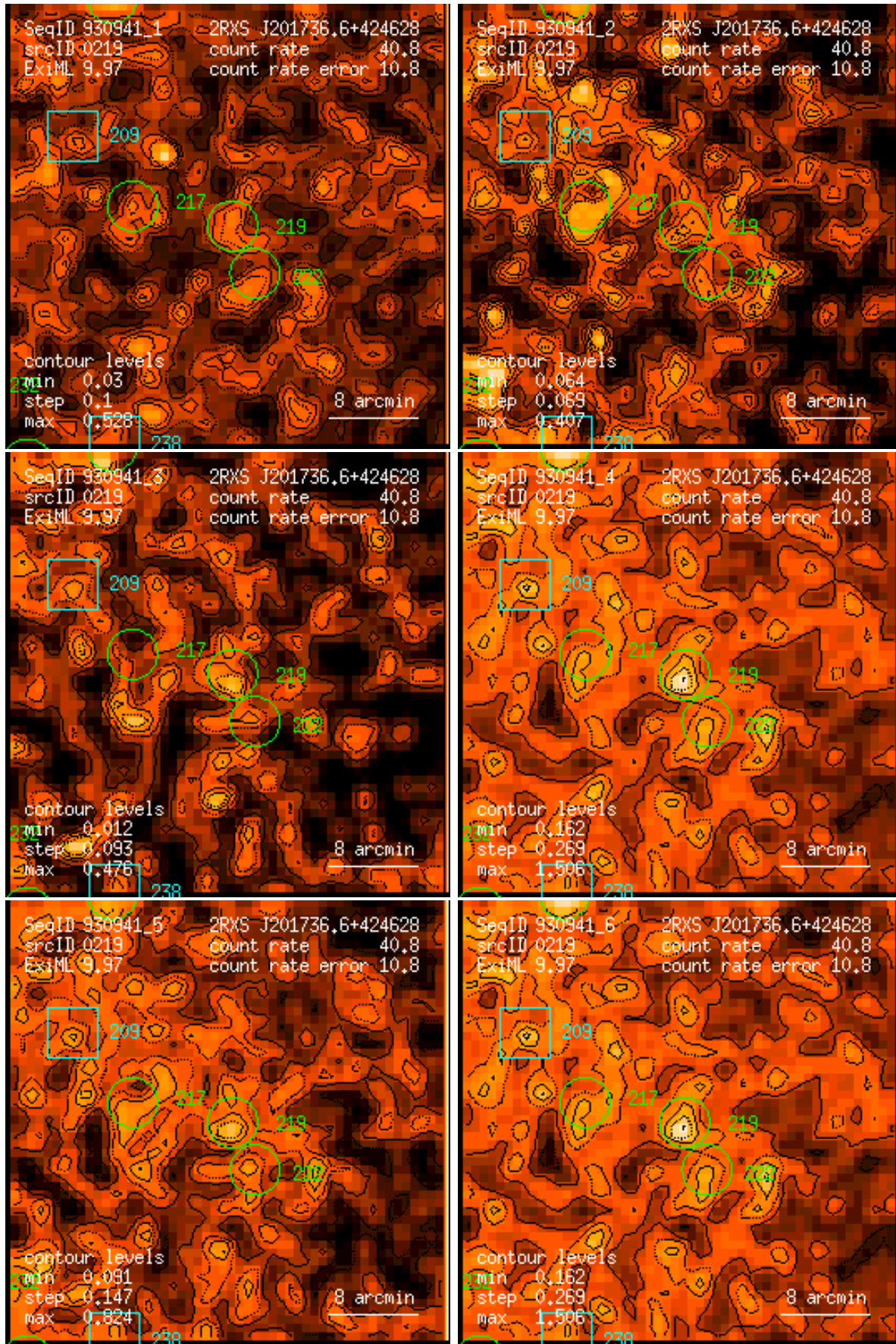
Figure 219: RASS 930941: detection 0219: band rate images, Gaussian filter: (1) PSPC channels 11 – 41, (2) 52 – 90, (3) 91 – 201, (4) 11 – 235, (5) 52 – 201, (6) 11 – 201. Broad band rates in counts/ks. Band rate contour levels in counts/ks/arcmin 2 .
