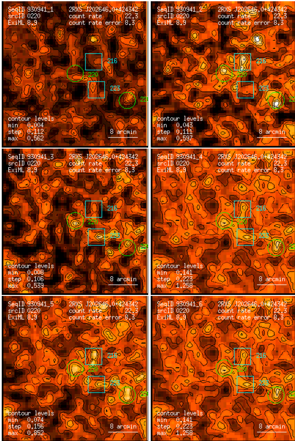
Figure 220: RASS 930941: detection 0220: band rate images, Gaussian filter: (1) PSPC channels 11 – 41, (2) 52 – 90, (3) 91 – 201, (4) 11 – 235, (5) 52 – 201, (6) 11 – 201. Broad band rates in counts/ks. Band rate contour levels in counts/ks/arcmin 2 .
