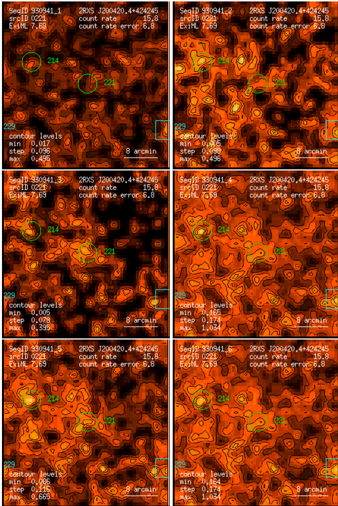
Figure 221: RASS 930941: detection 0221: band rate images, Gaussian filter: (1) PSPC channels 11 – 41, (2) 52 – 90, (3) 91 – 201, (4) 11 – 235, (5) 52 – 201, (6) 11 – 201. Broad band rates in counts/ks. Band rate contour levels in counts/ks/arcmin 2 .
