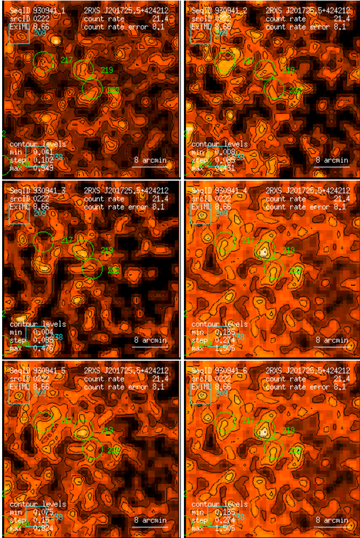
Figure 222: RASS 930941: detection 0222: band rate images, Gaussian filter: (1) PSPC channels 11 – 41, (2) 52 – 90, (3) 91 – 201, (4) 11 – 235, (5) 52 – 201, (6) 11 – 201. Broad band rates in counts/ks. Band rate contour levels in counts/ks/arcmin 2 .
