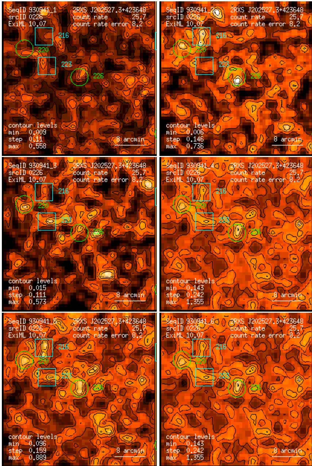
Figure 226: RASS 930941: detection 0226: band rate images, Gaussian filter: (1) PSPC channels 11 – 41, (2) 52 – 90, (3) 91 – 201, (4) 11 – 235, (5) 52 – 201, (6) 11 – 201. Broad band rates in counts/ks. Band rate contour levels in counts/ks/arcmin 2 .
