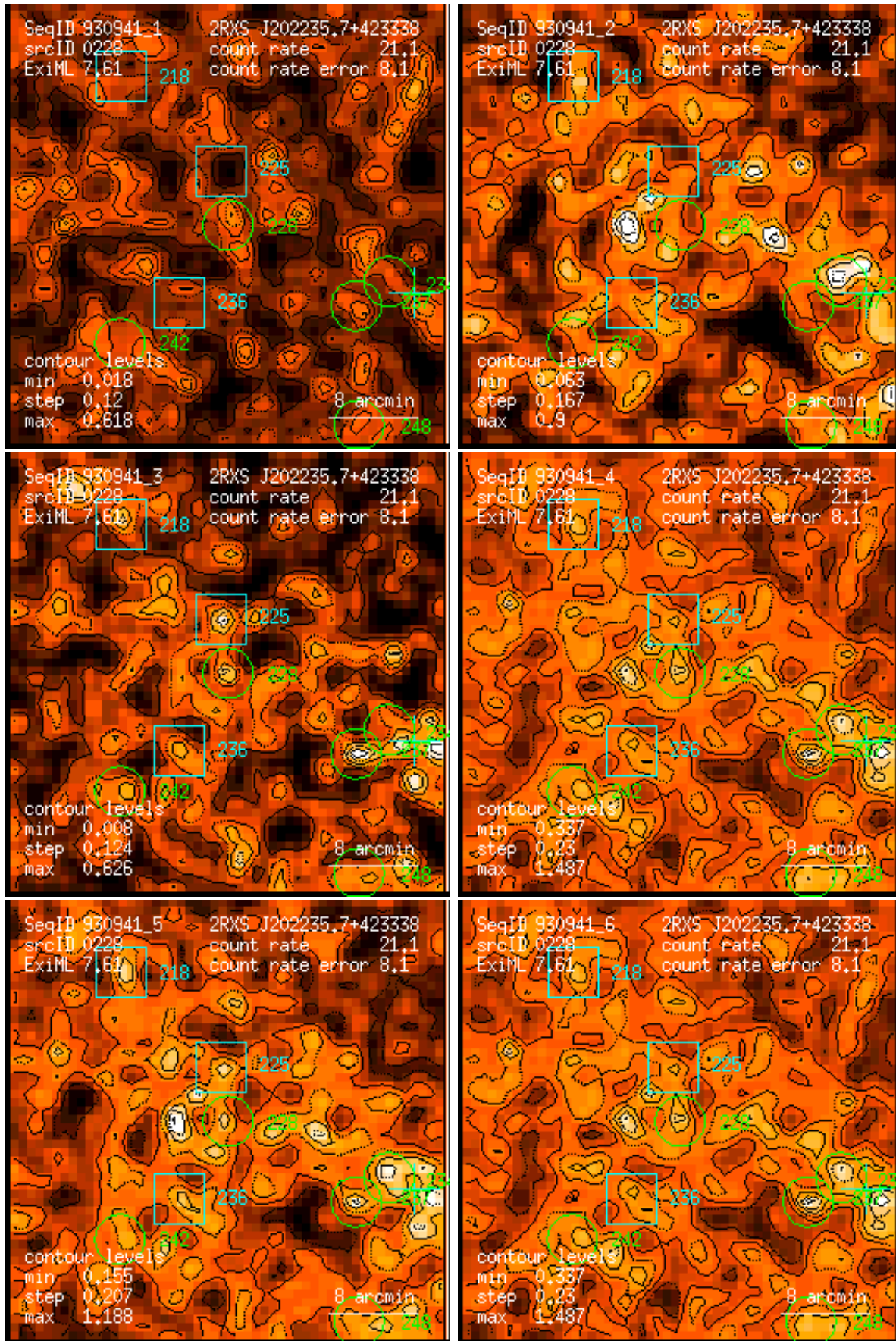
Figure 228: RASS 930941: detection 0228: band rate images, Gaussian filter: (1) PSPC channels 11 – 41, (2) 52 – 90, (3) 91 – 201, (4) 11 – 235, (5) 52 – 201, (6) 11 – 201. Broad band rates in counts/ks. Band rate contour levels in counts/ks/arcmin 2 .
