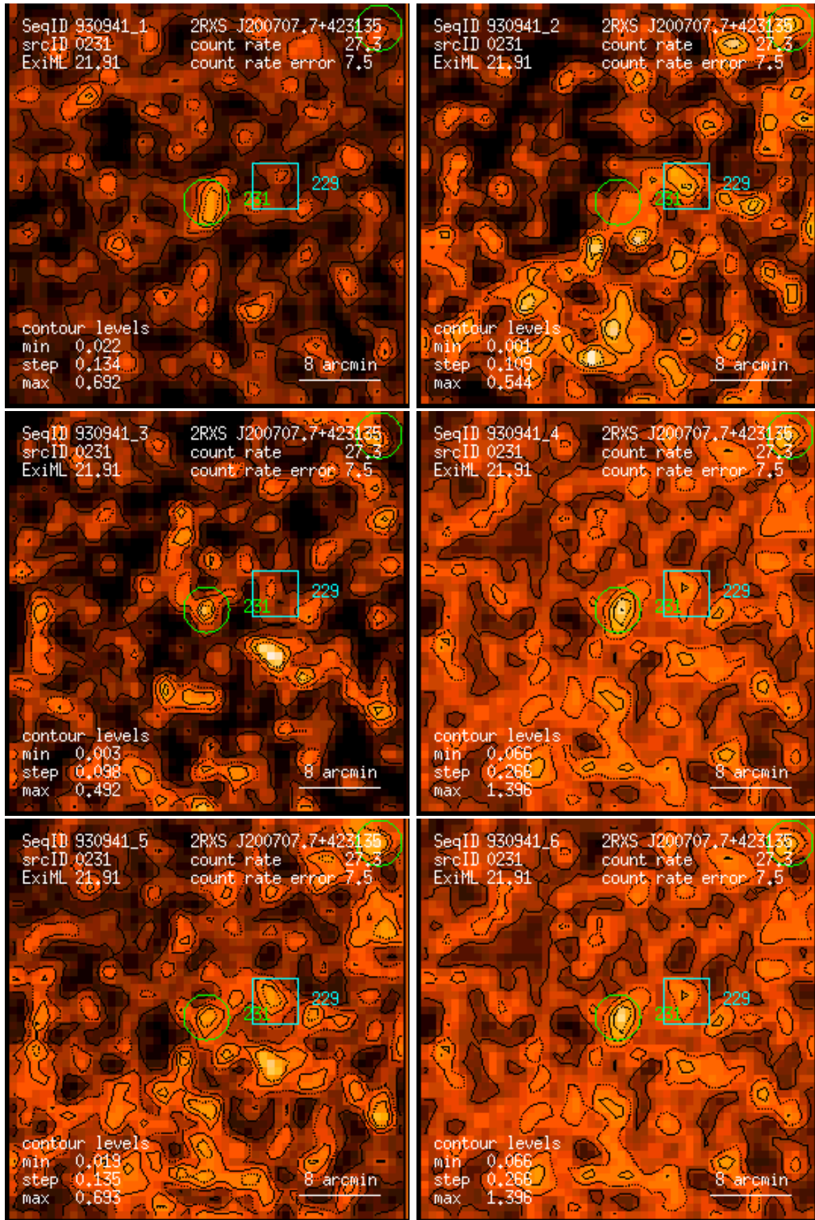
Figure 231: RASS 930941: detection 0231: band rate images, Gaussian filter: (1) PSPC channels 11 – 41, (2) 52 – 90, (3) 91 – 201, (4) 11 – 235, (5) 52 – 201, (6) 11 – 201. Broad band rates in counts/ks. Band rate contour levels in counts/ks/arcmin 2 .
