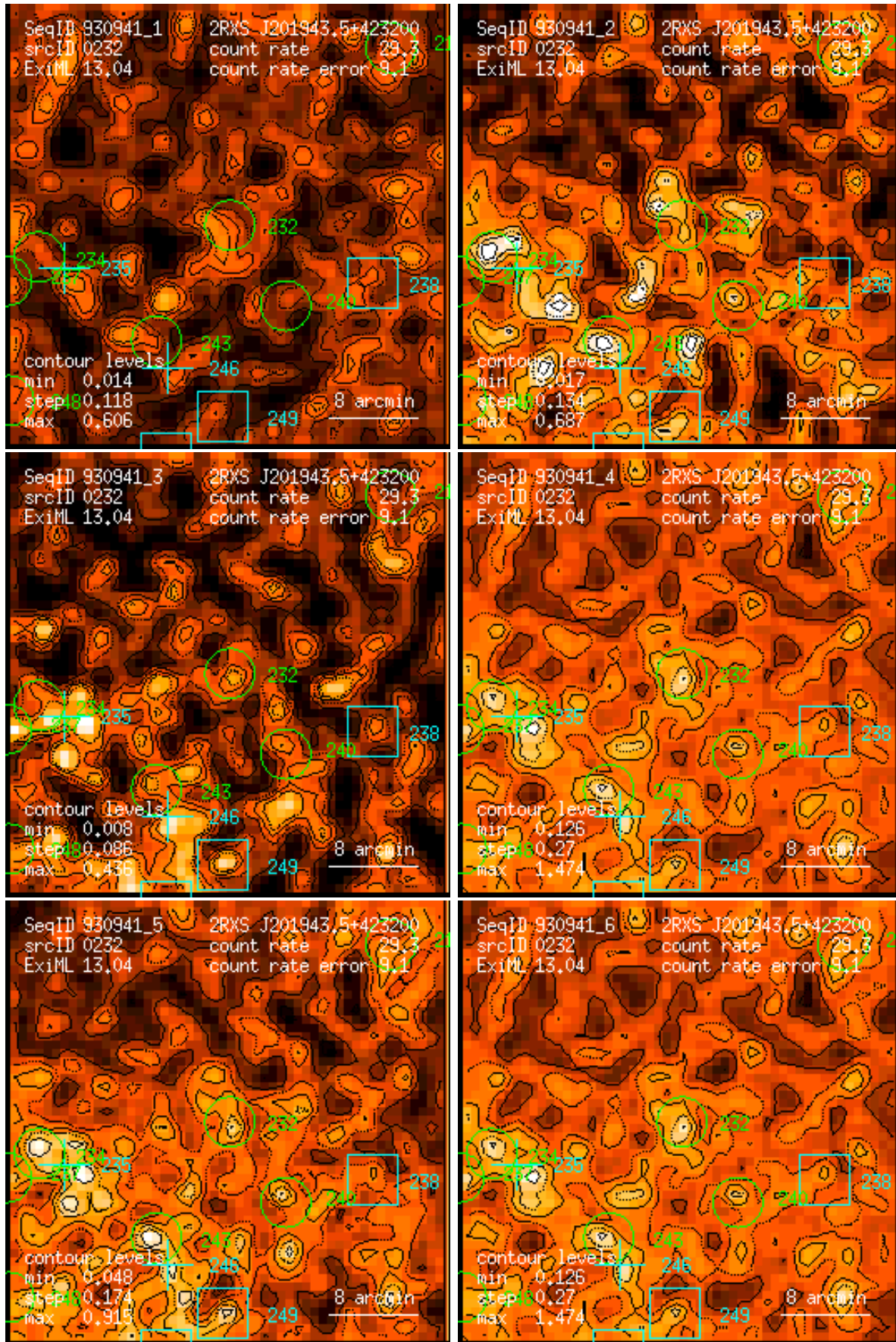
Figure 232: RASS 930941: detection 0232: band rate images, Gaussian filter: (1) PSPC channels 11 – 41, (2) 52 – 90, (3) 91 – 201, (4) 11 – 235, (5) 52 – 201, (6) 11 – 201. Broad band rates in counts/ks. Band rate contour levels in counts/ks/arcmin 2 .
