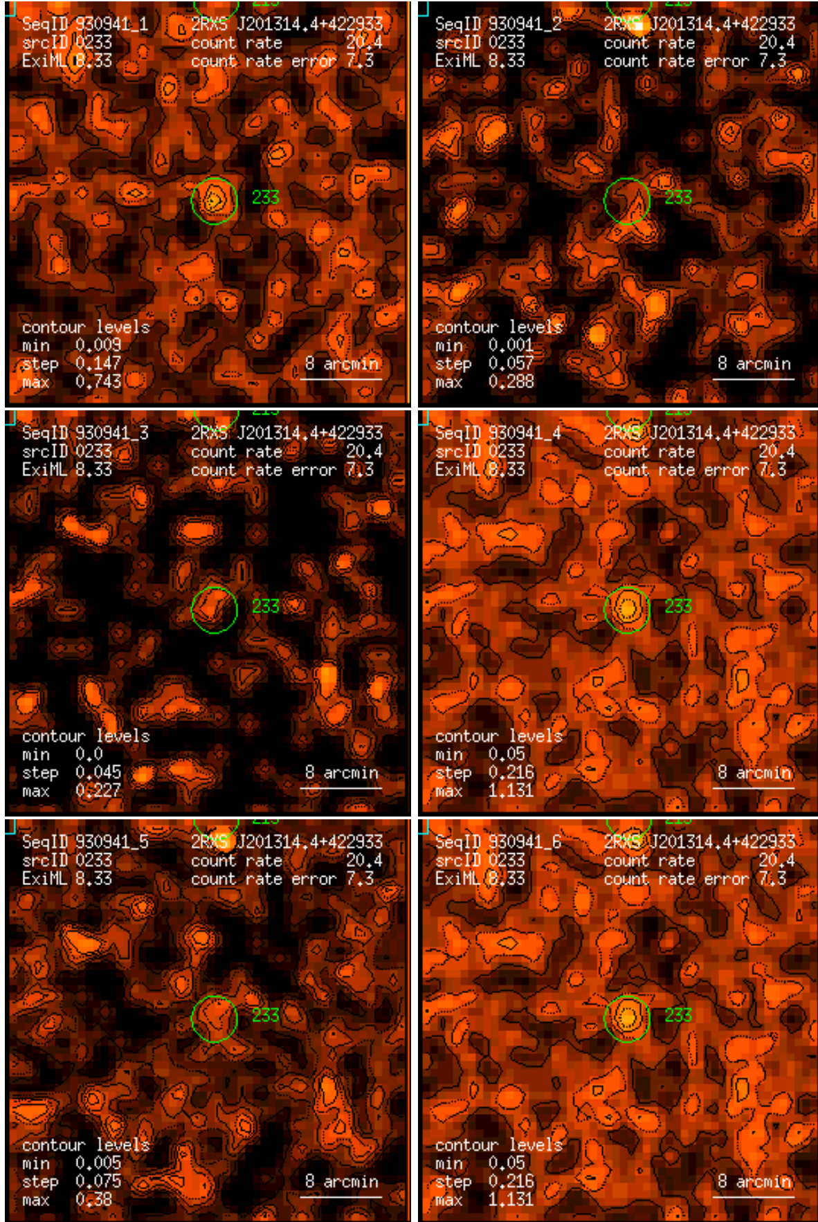
Figure 233: RASS 930941: detection 0233: band rate images, Gaussian filter: (1) PSPC channels 11 – 41, (2) 52 – 90, (3) 91 – 201, (4) 11 – 235, (5) 52 – 201, (6) 11 – 201. Broad band rates in counts/ks. Band rate contour levels in counts/ks/arcmin 2 .
