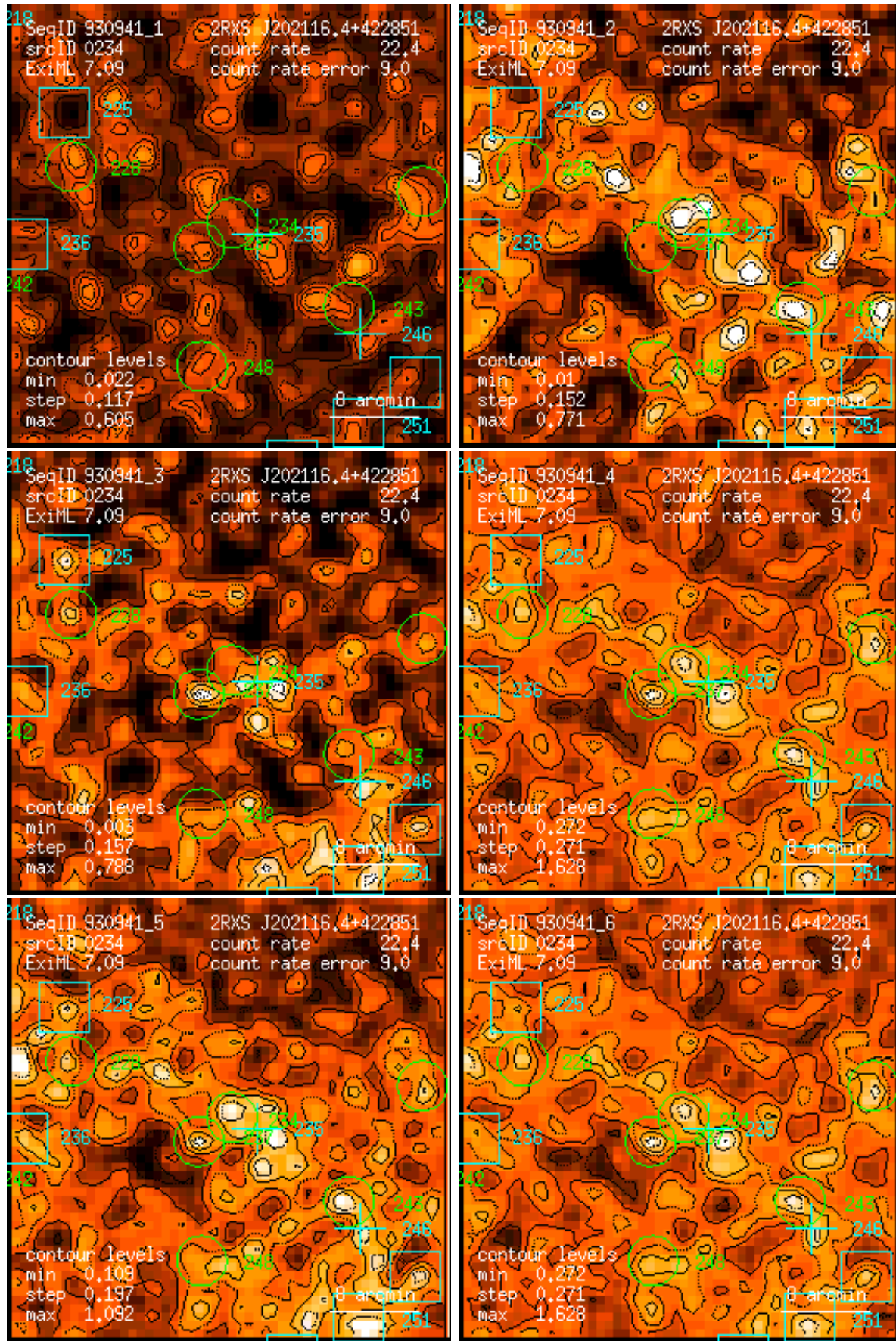
Figure 234: RASS 930941: detection 0234: band rate images, Gaussian filter: (1) PSPC channels 11 – 41, (2) 52 – 90, (3) 91 – 201, (4) 11 – 235, (5) 52 – 201, (6) 11 – 201. Broad band rates in counts/ks. Band rate contour levels in counts/ks/arcmin 2 .
