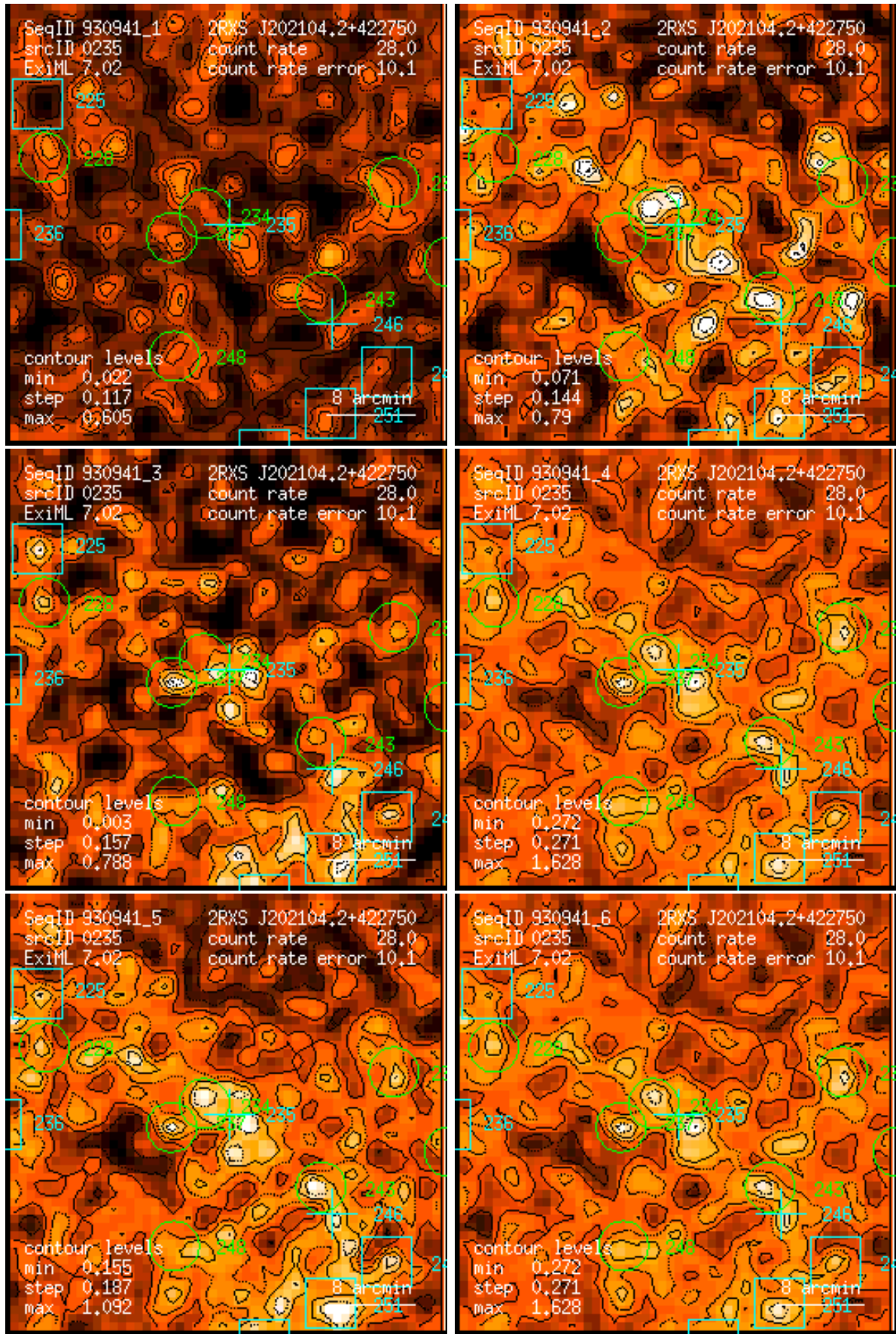
Figure 235: RASS 930941: detection 0235: band rate images, Gaussian filter: (1) PSPC channels 11 – 41, (2) 52 – 90, (3) 91 – 201, (4) 11 – 235, (5) 52 – 201, (6) 11 – 201. Broad band rates in counts/ks. Band rate contour levels in counts/ks/arcmin 2 .
