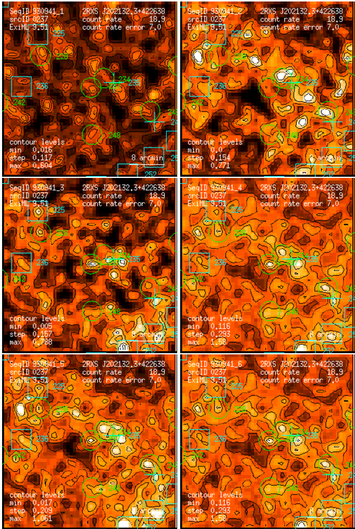
Figure 237: RASS 930941: detection 0237: band rate images, Gaussian filter: (1) PSPC channels 11 – 41, (2) 52 – 90, (3) 91 – 201, (4) 11 – 235, (5) 52 – 201, (6) 11 – 201. Broad band rates in counts/ks. Band rate contour levels in counts/ks/arcmin 2 .
