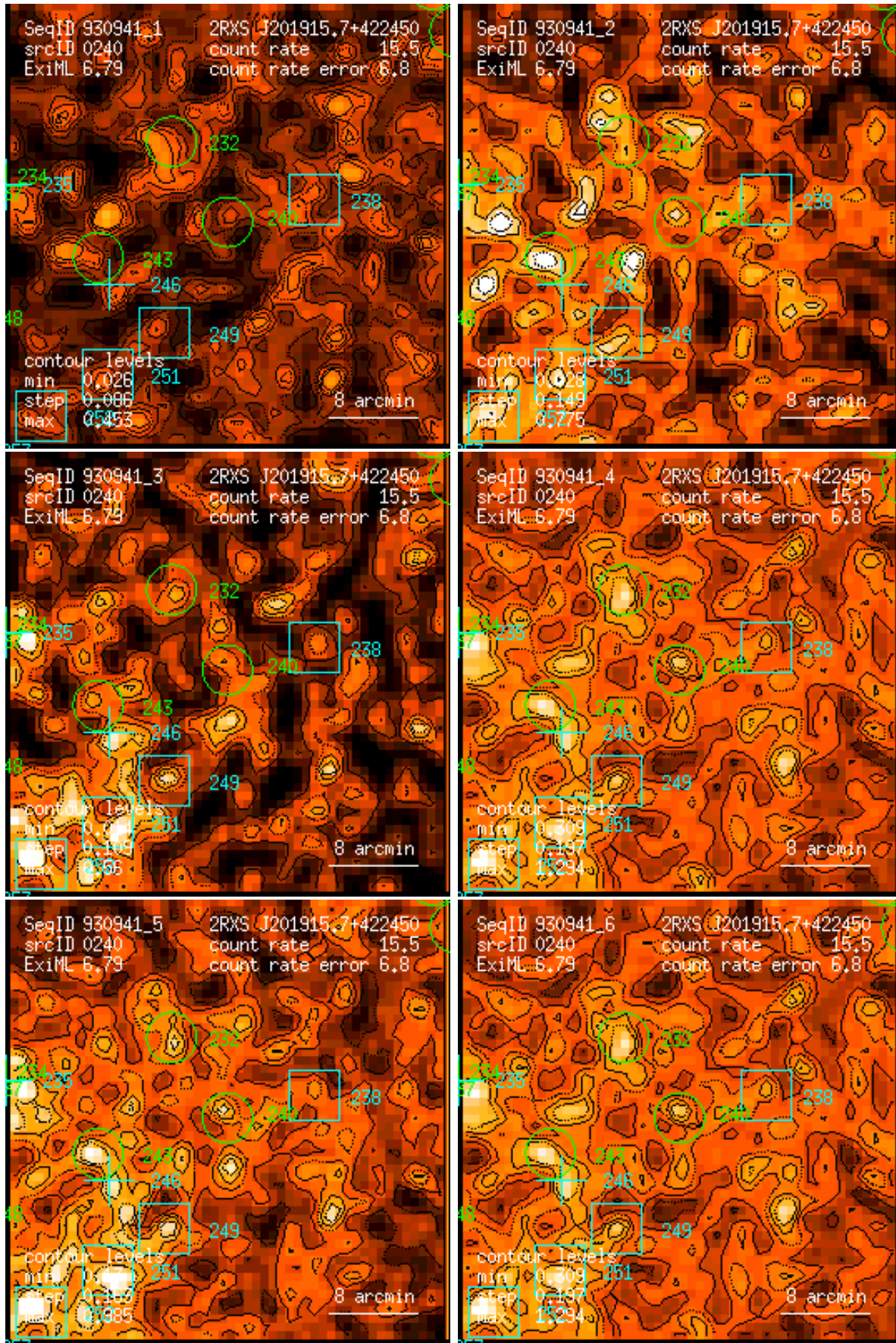
Figure 240: RASS 930941: detection 0240: band rate images, Gaussian filter: (1) PSPC channels 11 – 41, (2) 52 – 90, (3) 91 – 201, (4) 11 – 235, (5) 52 – 201, (6) 11 – 201. Broad band rates in counts/ks. Band rate contour levels in counts/ks/arcmin 2 .
