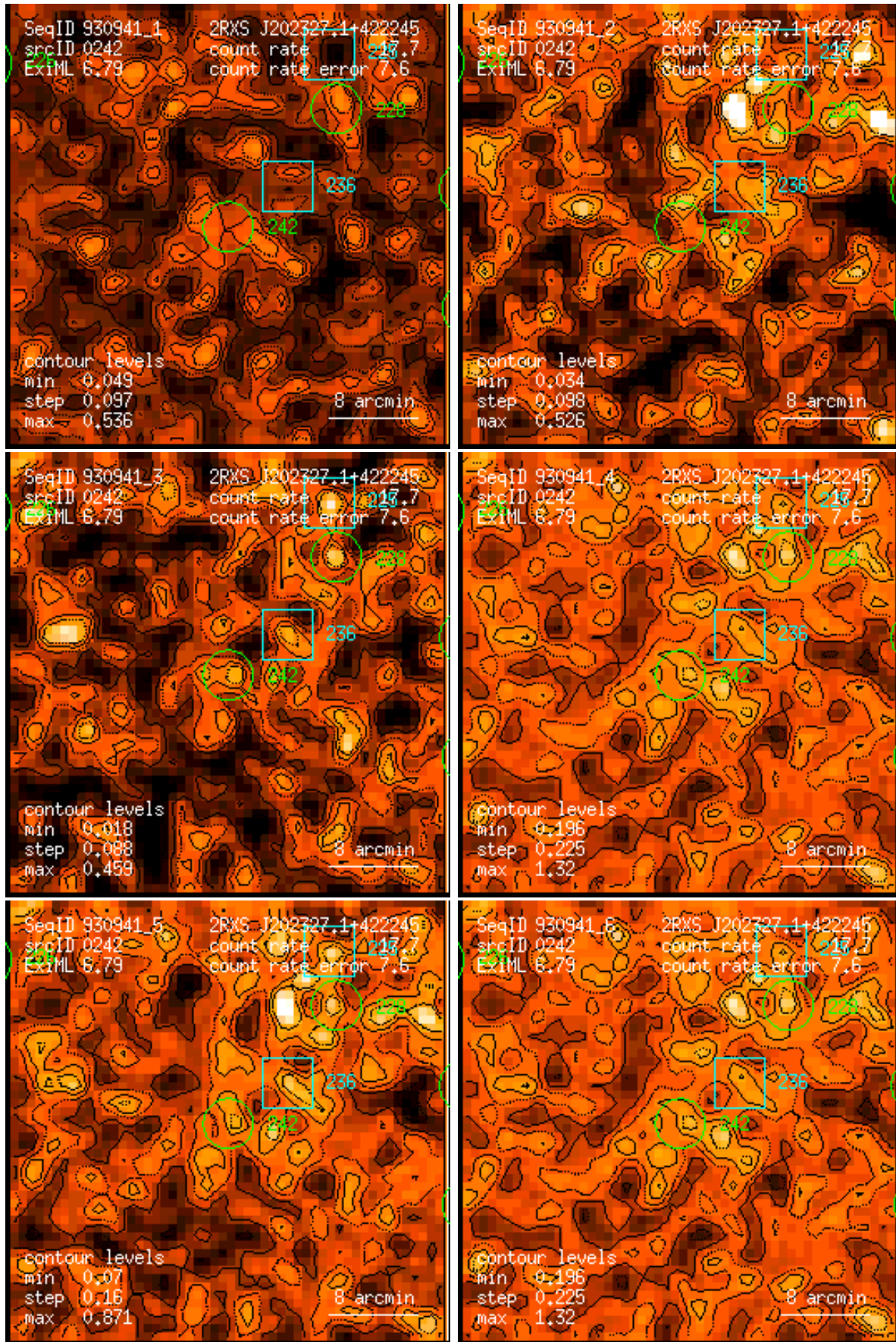
Figure 242: RASS 930941: detection 0242: band rate images, Gaussian filter: (1) PSPC channels 11 – 41, (2) 52 – 90, (3) 91 – 201, (4) 11 – 235, (5) 52 – 201, (6) 11 – 201. Broad band rates in counts/ks. Band rate contour levels in counts/ks/arcmin 2 .
