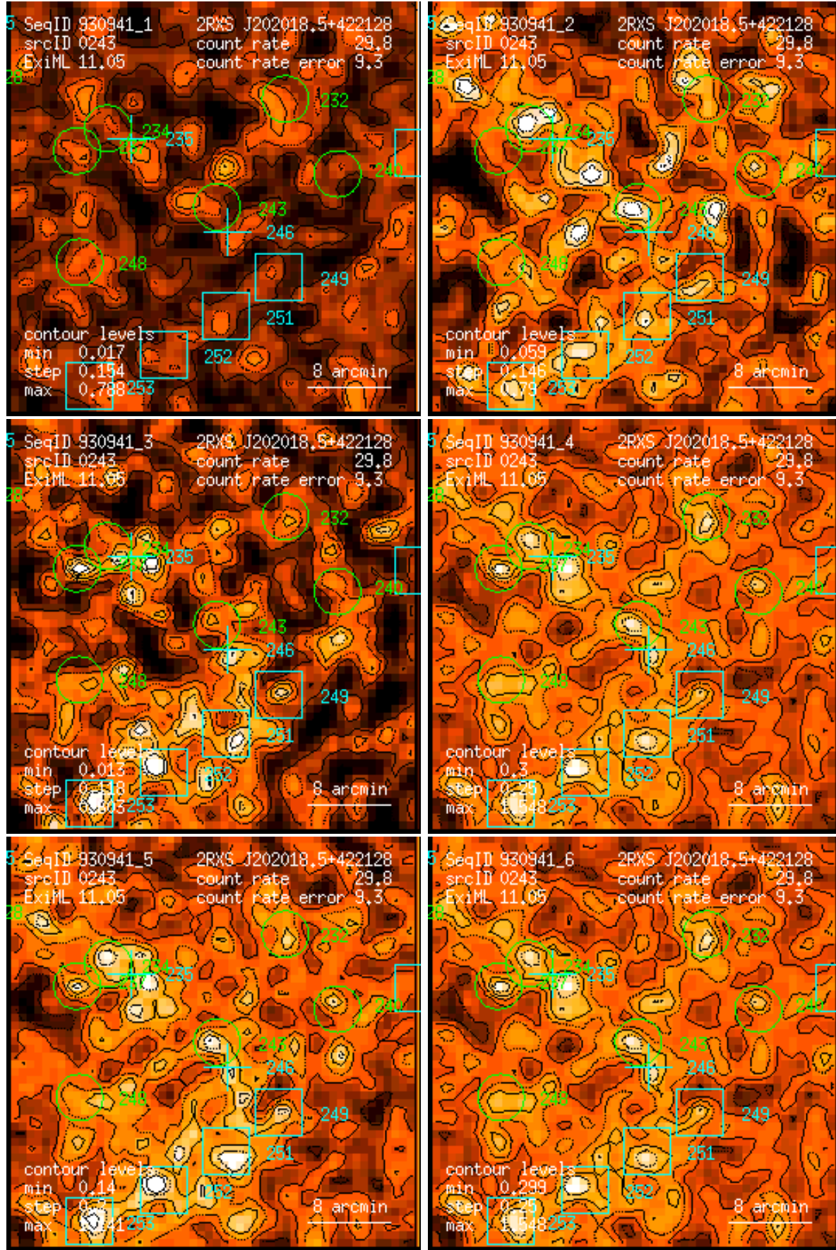
Figure 243: RASS 930941: detection 0243: band rate images, Gaussian filter: (1) PSPC channels 11 – 41, (2) 52 – 90, (3) 91 – 201, (4) 11 – 235, (5) 52 – 201, (6) 11 – 201. Broad band rates in counts/ks. Band rate contour levels in counts/ks/arcmin 2 .
