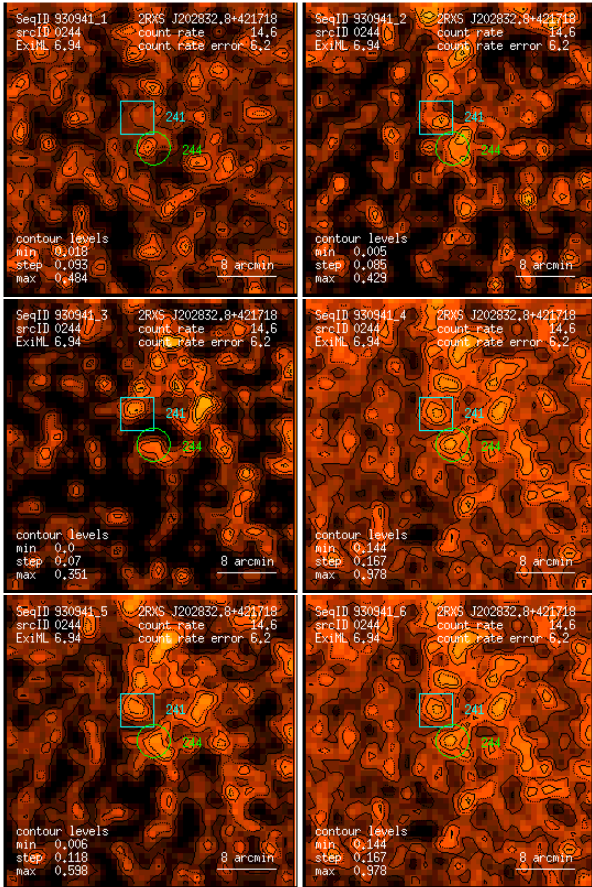
Figure 244: RASS 930941: detection 0244: band rate images, Gaussian filter: (1) PSPC channels 11 – 41, (2) 52 – 90, (3) 91 – 201, (4) 11 – 235, (5) 52 – 201, (6) 11 – 201. Broad band rates in counts/ks. Band rate contour levels in counts/ks/arcmin 2 .
