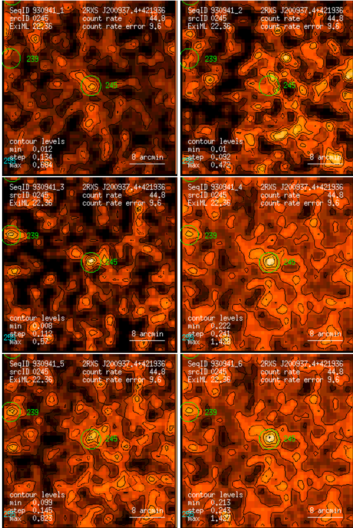
Figure 245: RASS 930941: detection 0245: band rate images, Gaussian filter: (1) PSPC channels 11 – 41, (2) 52 – 90, (3) 91 – 201, (4) 11 – 235, (5) 52 – 201, (6) 11 – 201. Broad band rates in counts/ks. Band rate contour levels in counts/ks/arcmin 2 .
