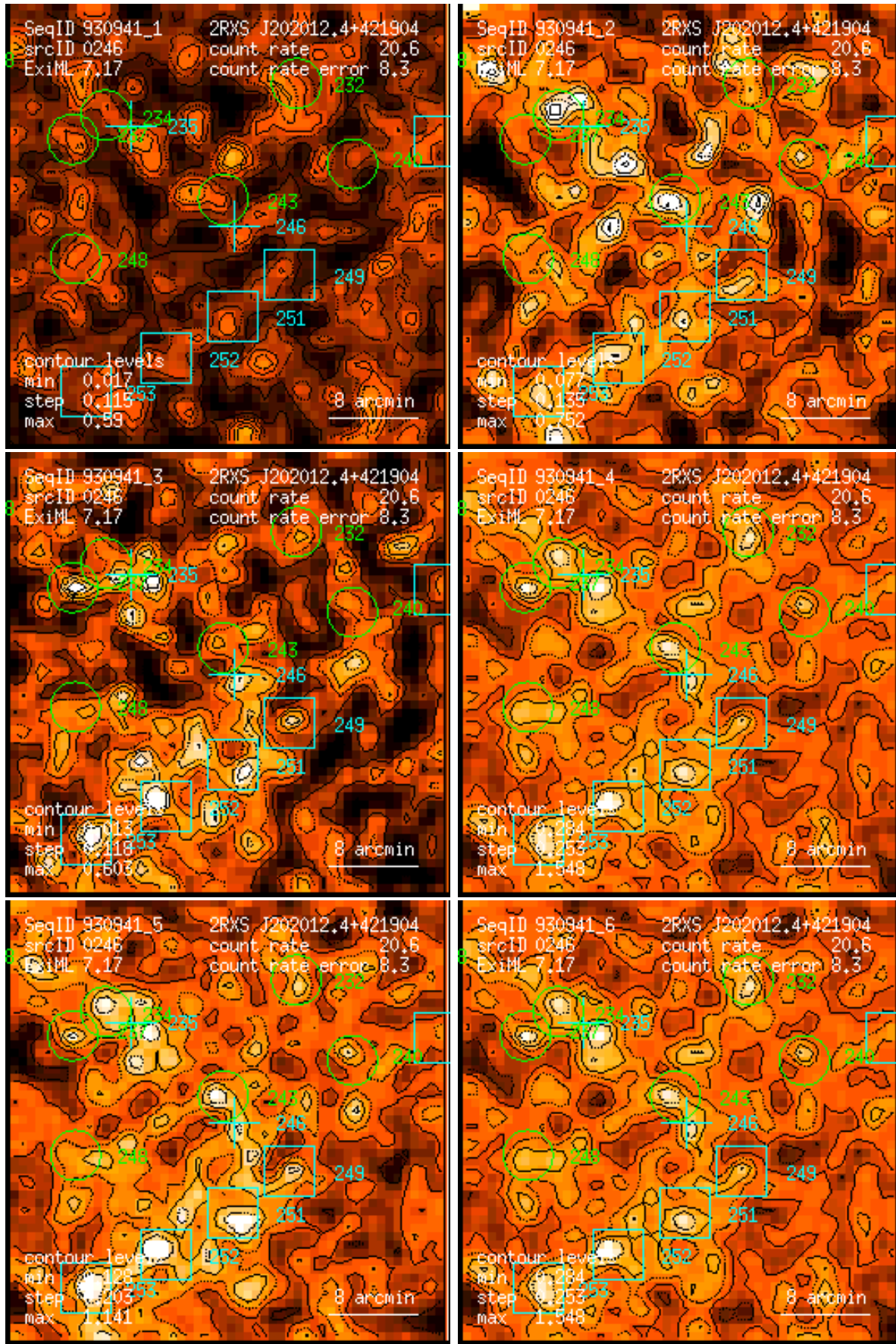
Figure 246: RASS 930941: detection 0246: band rate images, Gaussian filter: (1) PSPC channels 11 – 41, (2) 52 – 90, (3) 91 – 201, (4) 11 – 235, (5) 52 – 201, (6) 11 – 201. Broad band rates in counts/ks. Band rate contour levels in counts/ks/arcmin 2 .
