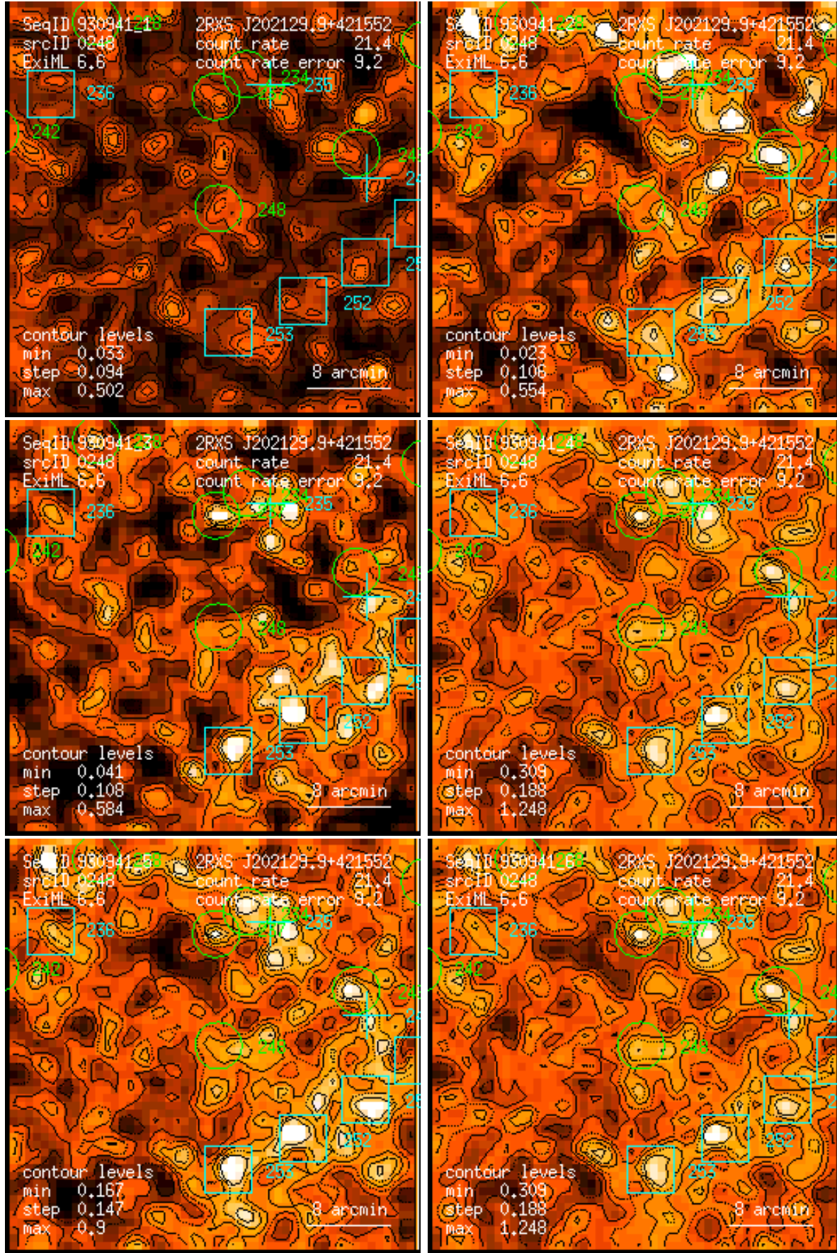
Figure 248: RASS 930941: detection 0248: band rate images, Gaussian filter: (1) PSPC channels 11 – 41, (2) 52 – 90, (3) 91 – 201, (4) 11 – 235, (5) 52 – 201, (6) 11 – 201. Broad band rates in counts/ks. Band rate contour levels in counts/ks/arcmin 2 .
