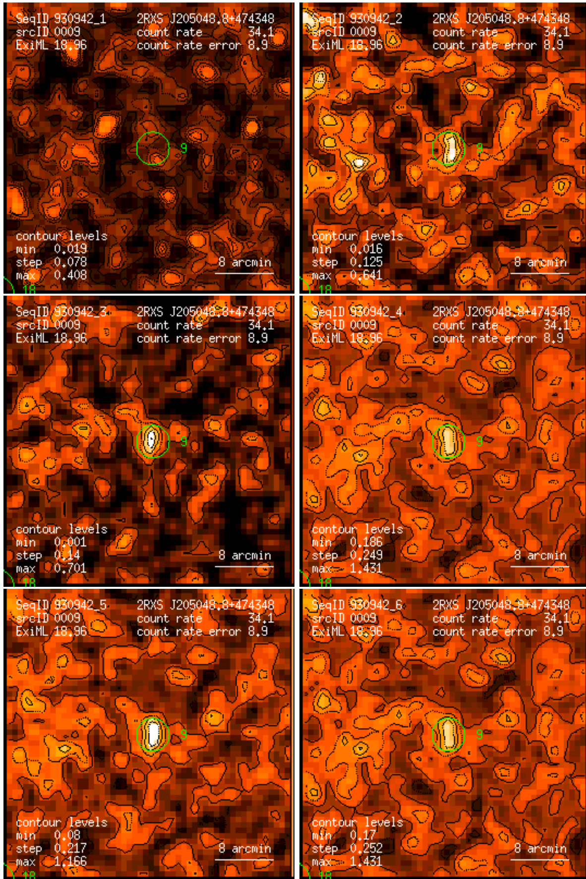
Figure 9: RASS 930942: detection 0009: band rate images, Gaussian filter: (1) PSPC channels 11 – 41, (2) 52 – 90, (3) 91 – 201, (4) 11 – 235, (5) 52 – 201, (6) 11 – 201. Broad band rates in counts/ks. Band rate contour levels in counts/ks/arcmin 2 .
