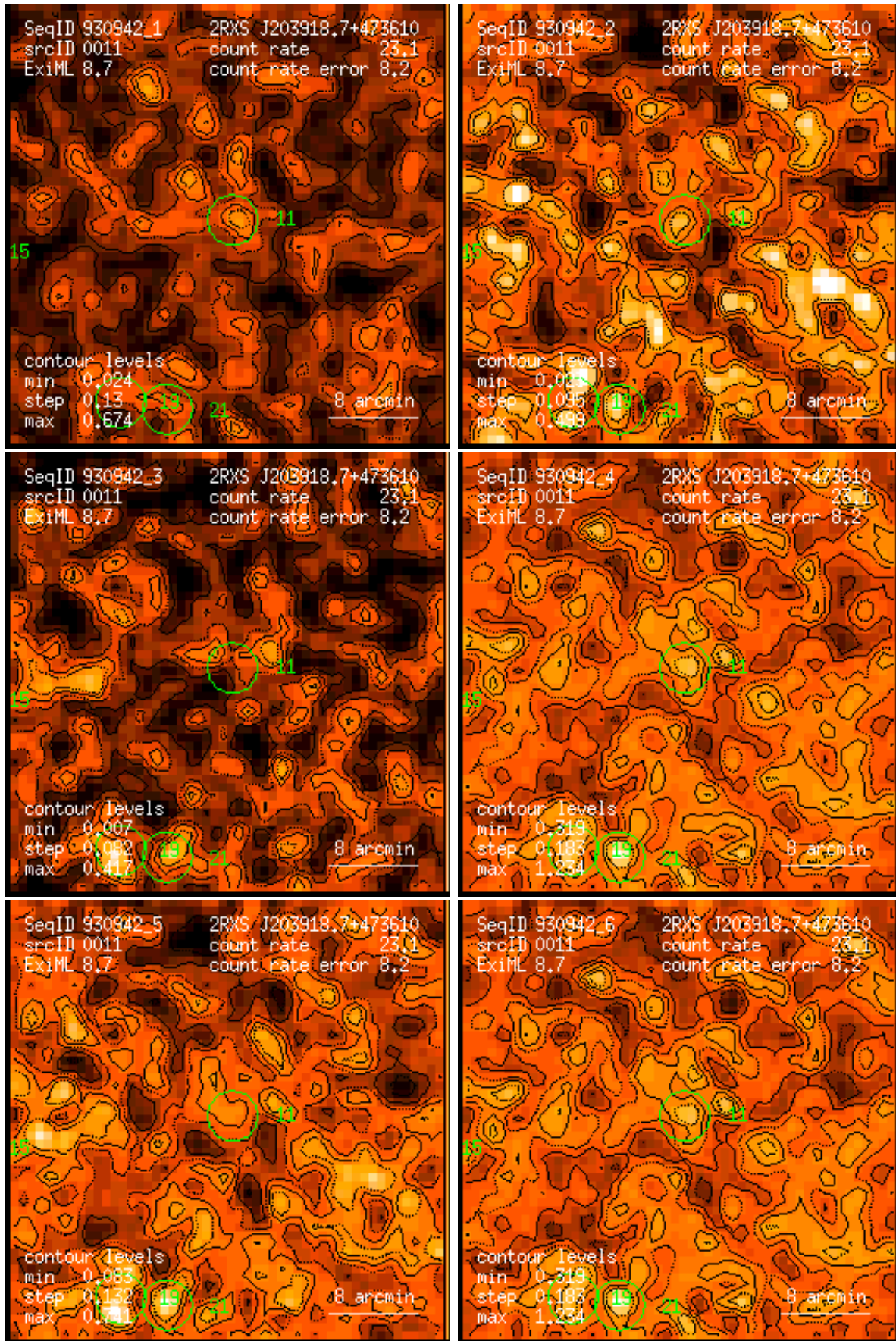
Figure 11: RASS 930942: detection 0011: band rate images, Gaussian filter: (1) PSPC channels 11 – 41, (2) 52 – 90, (3) 91 – 201, (4) 11 – 235, (5) 52 – 201, (6) 11 – 201. Broad band rates in counts/ks. Band rate contour levels in counts/ks/arcmin 2 .
