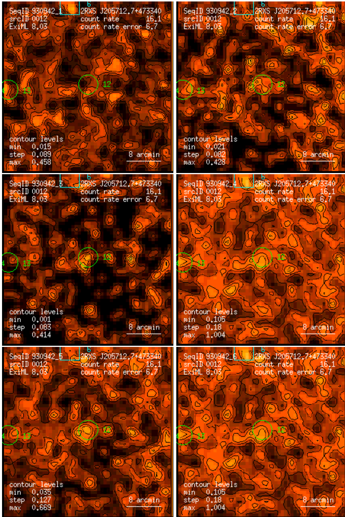
Figure 12: RASS 930942: detection 0012: band rate images, Gaussian filter: (1) PSPC channels 11 – 41, (2) 52 – 90, (3) 91 – 201, (4) 11 – 235, (5) 52 – 201, (6) 11 – 201. Broad band rates in counts/ks. Band rate contour levels in counts/ks/arcmin 2 .
