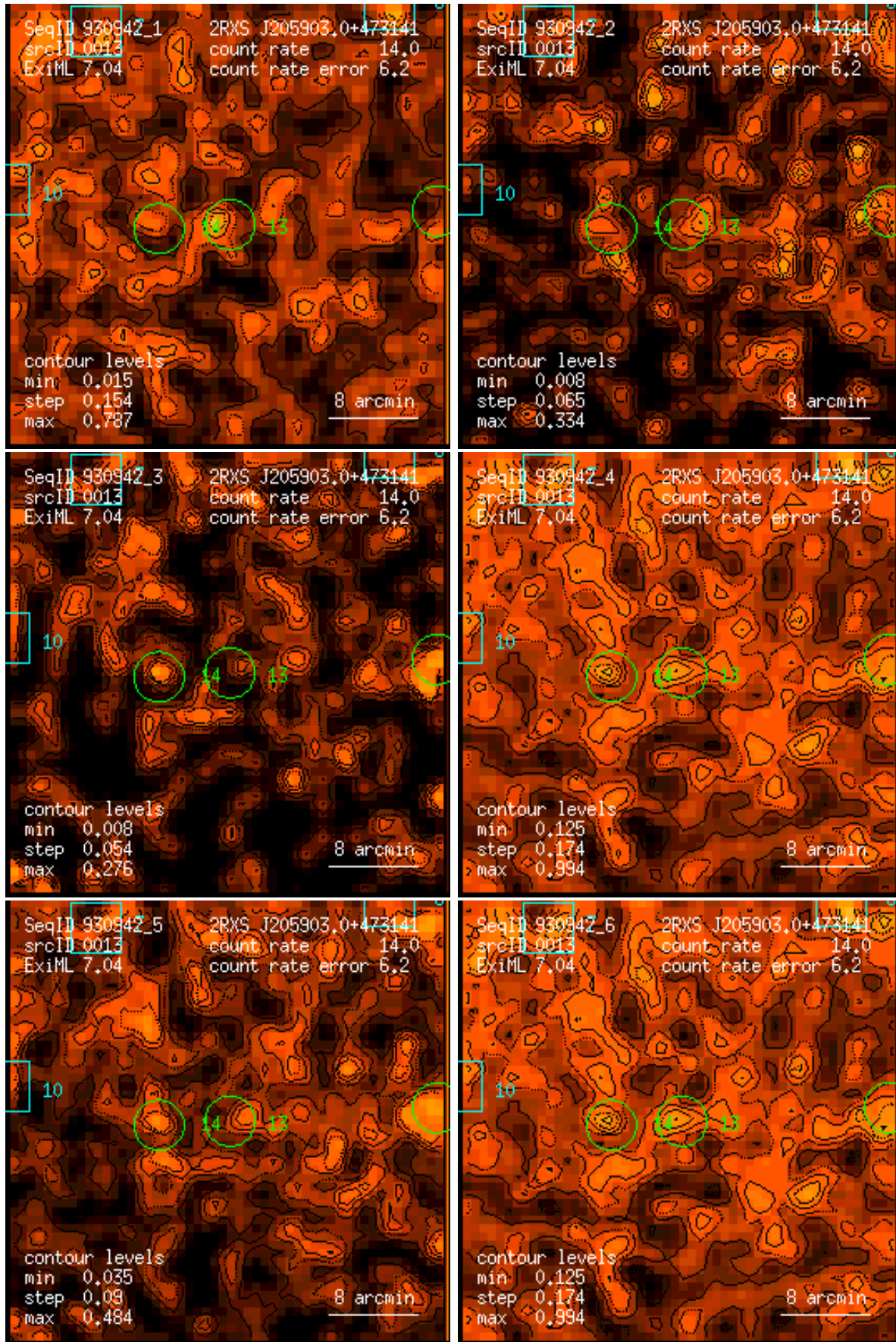
Figure 13: RASS 930942: detection 0013: band rate images, Gaussian filter: (1) PSPC channels 11 – 41, (2) 52 – 90, (3) 91 – 201, (4) 11 – 235, (5) 52 – 201, (6) 11 – 201. Broad band rates in counts/ks. Band rate contour levels in counts/ks/arcmin 2 .
