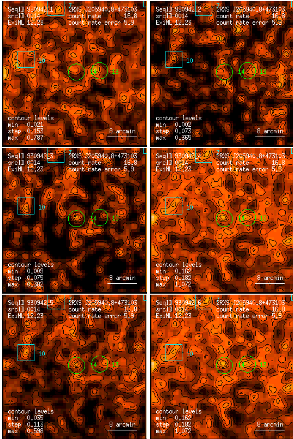
Figure 14: RASS 930942: detection 0014: band rate images, Gaussian filter: (1) PSPC channels 11 – 41, (2) 52 – 90, (3) 91 – 201, (4) 11 – 235, (5) 52 – 201, (6) 11 – 201. Broad band rates in counts/ks. Band rate contour levels in counts/ks/arcmin 2 .
