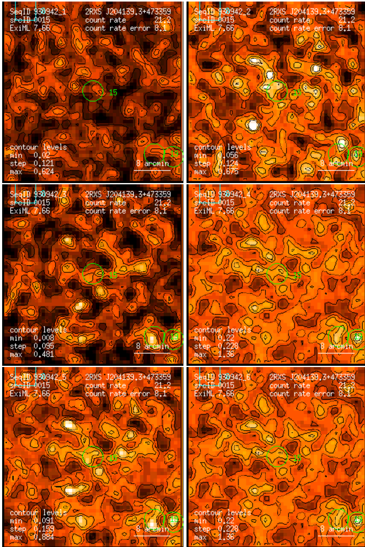
Figure 15: RASS 930942: detection 0015: band rate images, Gaussian filter: (1) PSPC channels 11 – 41, (2) 52 – 90, (3) 91 – 201, (4) 11 – 235, (5) 52 – 201, (6) 11 – 201. Broad band rates in counts/ks. Band rate contour levels in counts/ks/arcmin 2 .
