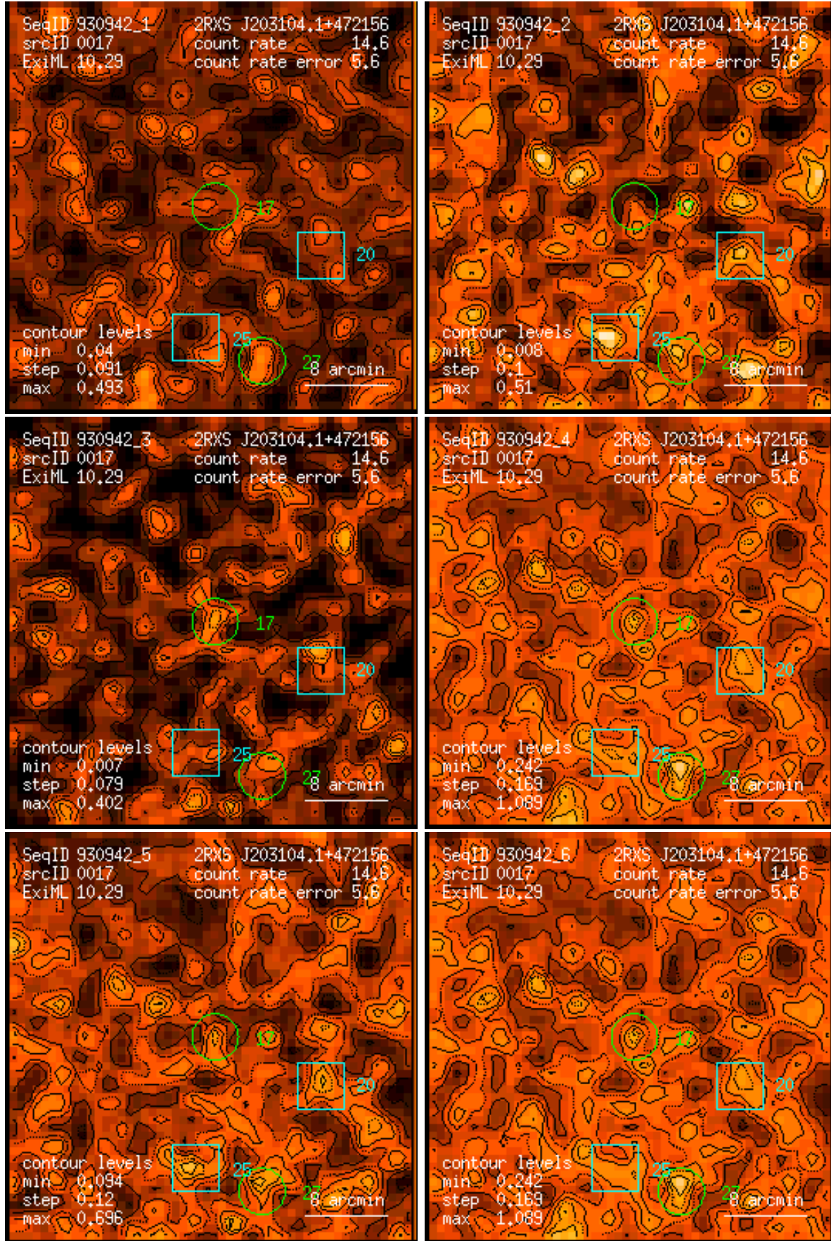
Figure 17: RASS 930942: detection 0017: band rate images, Gaussian filter: (1) PSPC channels 11 – 41, (2) 52 – 90, (3) 91 – 201, (4) 11 – 235, (5) 52 – 201, (6) 11 – 201. Broad band rates in counts/ks. Band rate contour levels in counts/ks/arcmin 2 .
