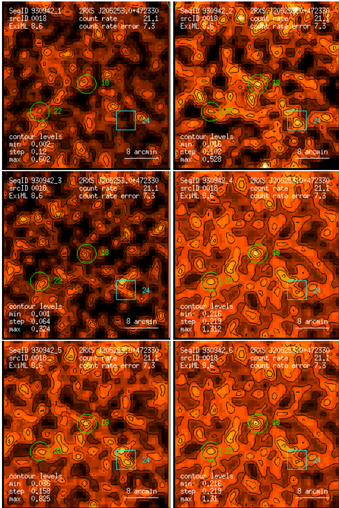
Figure 18: RASS 930942: detection 0018: band rate images, Gaussian filter: (1) PSPC channels 11 – 41, (2) 52 – 90, (3) 91 – 201, (4) 11 – 235, (5) 52 – 201, (6) 11 – 201. Broad band rates in counts/ks. Band rate contour levels in counts/ks/arcmin 2 .
