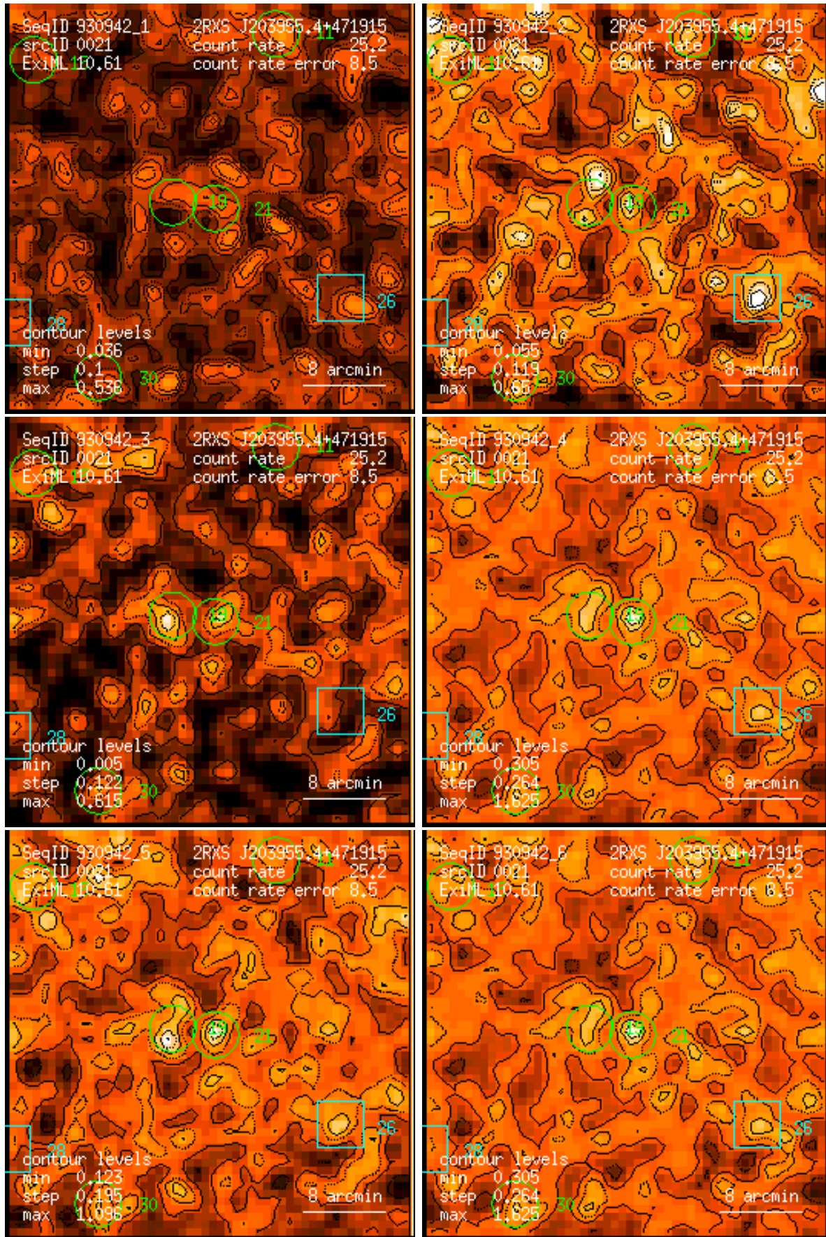
Figure 21: RASS 930942: detection 0021: band rate images, Gaussian filter: (1) PSPC channels 11 – 41, (2) 52 – 90, (3) 91 – 201, (4) 11 – 235, (5) 52 – 201, (6) 11 – 201. Broad band rates in counts/ks. Band rate contour levels in counts/ks/arcmin 2 .
