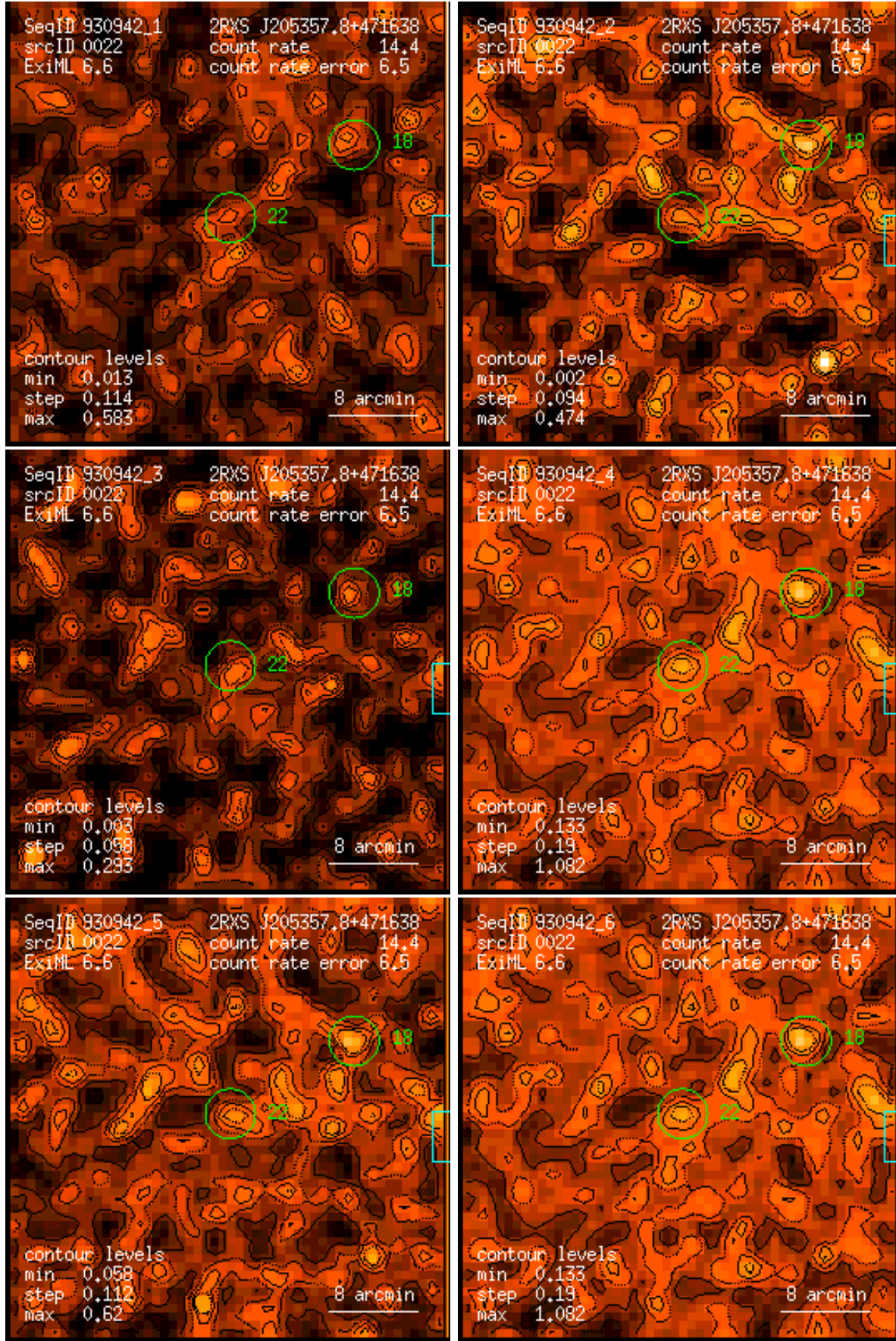
Figure 22: RASS 930942: detection 0022: band rate images, Gaussian filter: (1) PSPC channels 11 – 41, (2) 52 – 90, (3) 91 – 201, (4) 11 – 235, (5) 52 – 201, (6) 11 – 201. Broad band rates in counts/ks. Band rate contour levels in counts/ks/arcmin 2 .
