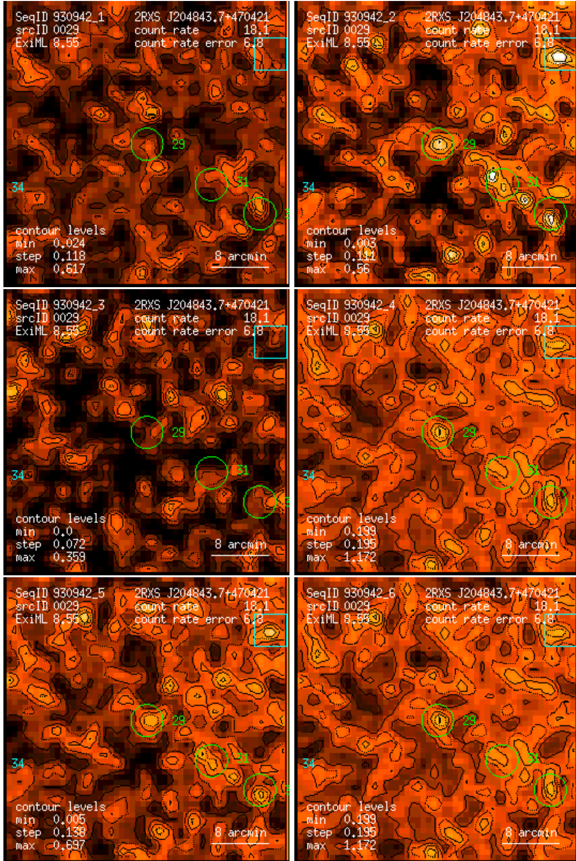
Figure 29: RASS 930942: detection 0029: band rate images, Gaussian filter: (1) PSPC channels 11 – 41, (2) 52 – 90, (3) 91 – 201, (4) 11 – 235, (5) 52 – 201, (6) 11 – 201. Broad band rates in counts/ks. Band rate contour levels in counts/ks/arcmin 2 .
