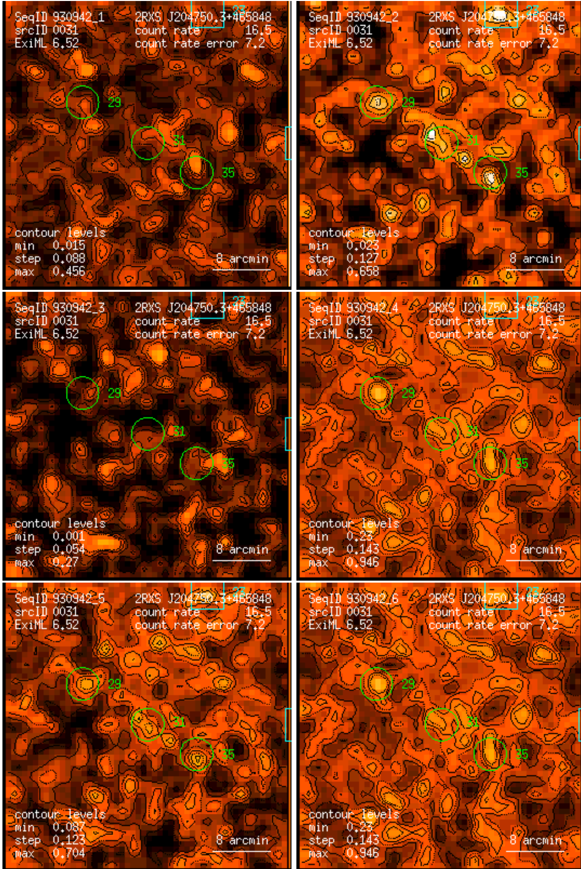
Figure 31: RASS 930942: detection 0031: band rate images, Gaussian filter: (1) PSPC channels 11 – 41, (2) 52 – 90, (3) 91 – 201, (4) 11 – 235, (5) 52 – 201, (6) 11 – 201. Broad band rates in counts/ks. Band rate contour levels in counts/ks/arcmin 2 .
