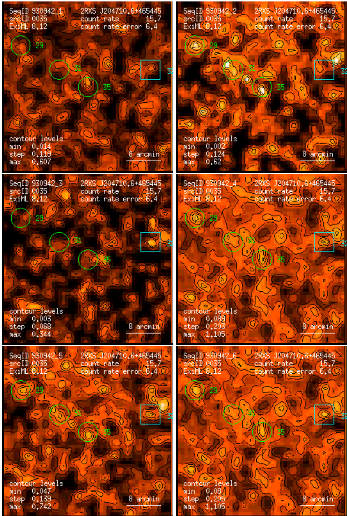
Figure 35: RASS 930942: detection 0035: band rate images, Gaussian filter: (1) PSPC channels 11 – 41, (2) 52 – 90, (3) 91 – 201, (4) 11 – 235, (5) 52 – 201, (6) 11 – 201. Broad band rates in counts/ks. Band rate contour levels in counts/ks/arcmin 2 .
