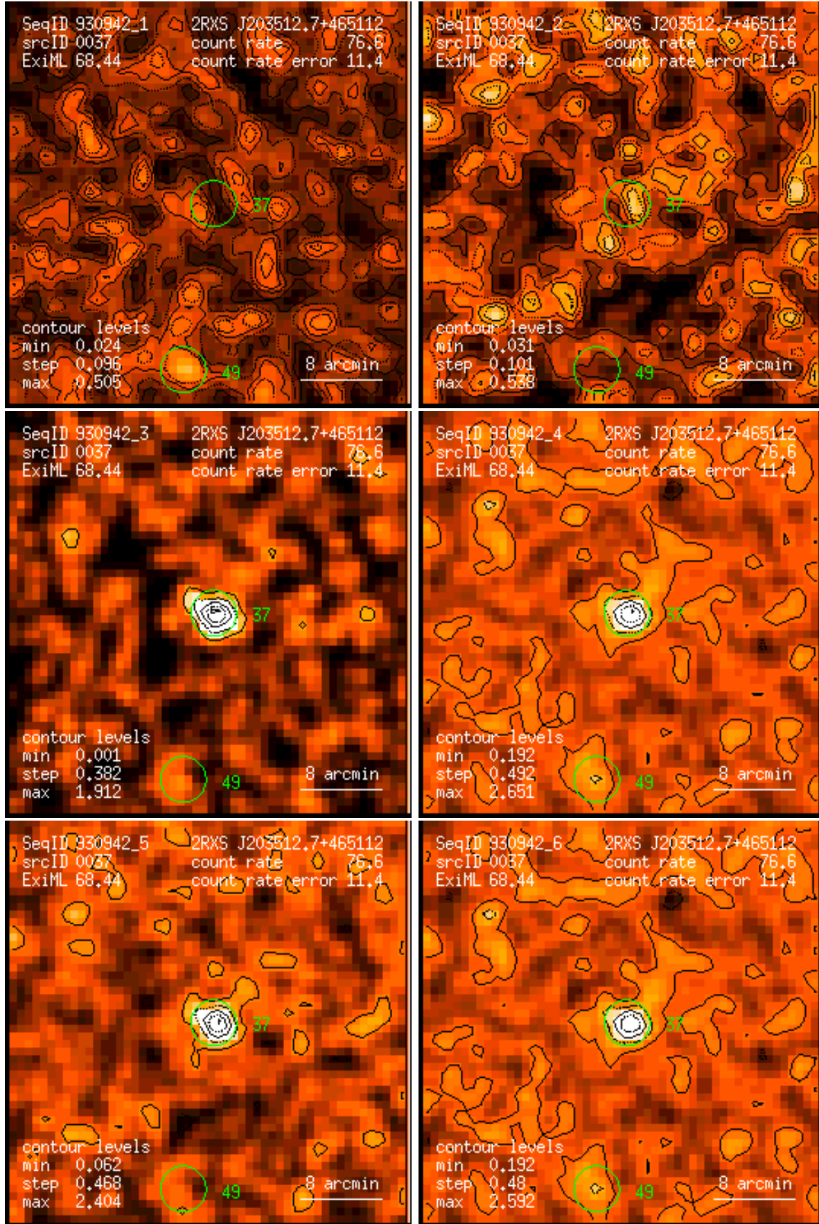
Figure 37: RASS 930942: detection 0037: band rate images, Gaussian filter: (1) PSPC channels 11 – 41, (2) 52 – 90, (3) 91 – 201, (4) 11 – 235, (5) 52 – 201, (6) 11 – 201. Broad band rates in counts/ks. Band rate contour levels in counts/ks/arcmin 2 .
