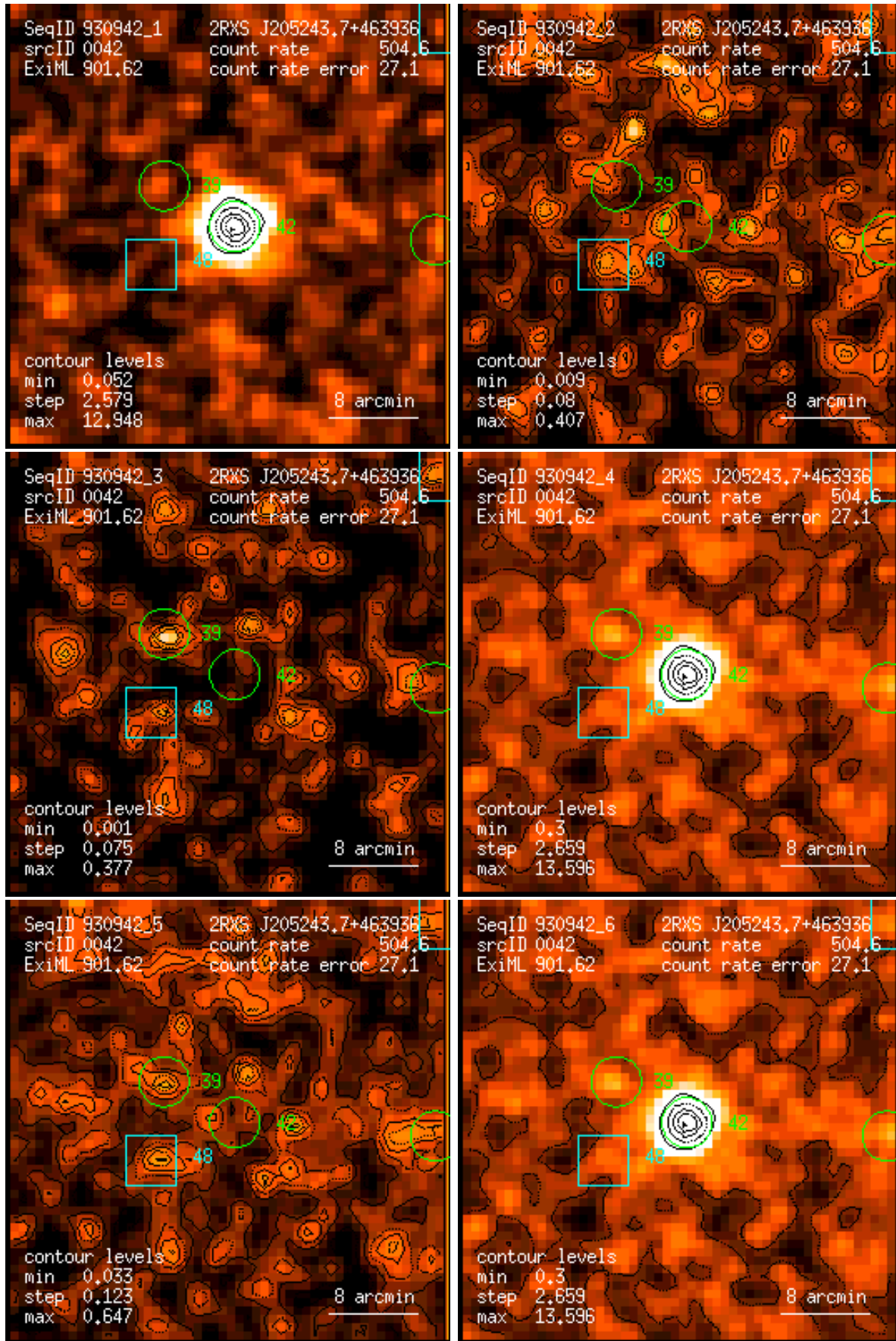
Figure 42: RASS 930942: detection 0042: band rate images, Gaussian filter: (1) PSPC channels 11 – 41, (2) 52 – 90, (3) 91 – 201, (4) 11 – 235, (5) 52 – 201, (6) 11 – 201. Broad band rates in counts/ks. Band rate contour levels in counts/ks/arcmin 2 .
