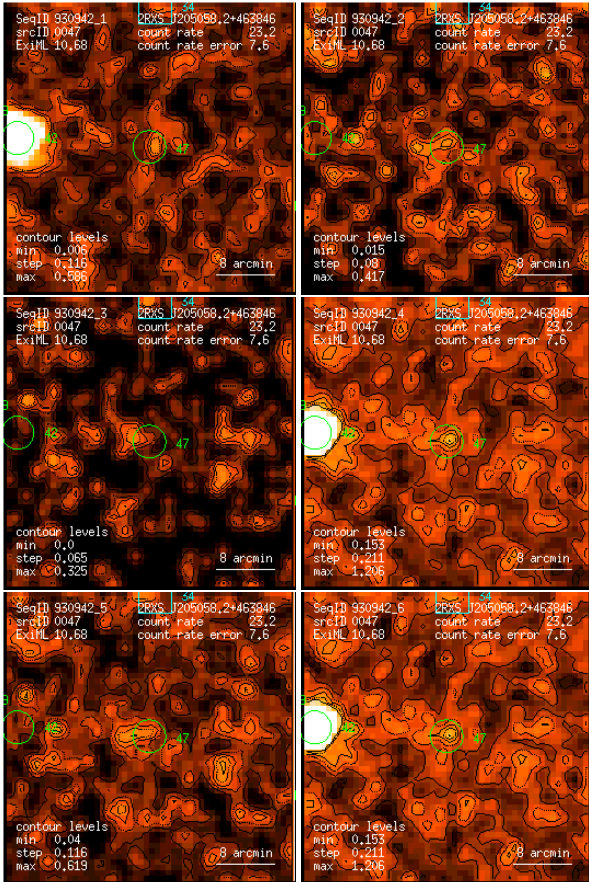
Figure 47: RASS 930942: detection 0047: band rate images, Gaussian filter: (1) PSPC channels 11 – 41, (2) 52 – 90, (3) 91 – 201, (4) 11 – 235, (5) 52 – 201, (6) 11 – 201. Broad band rates in counts/ks. Band rate contour levels in counts/ks/arcmin 2 .
