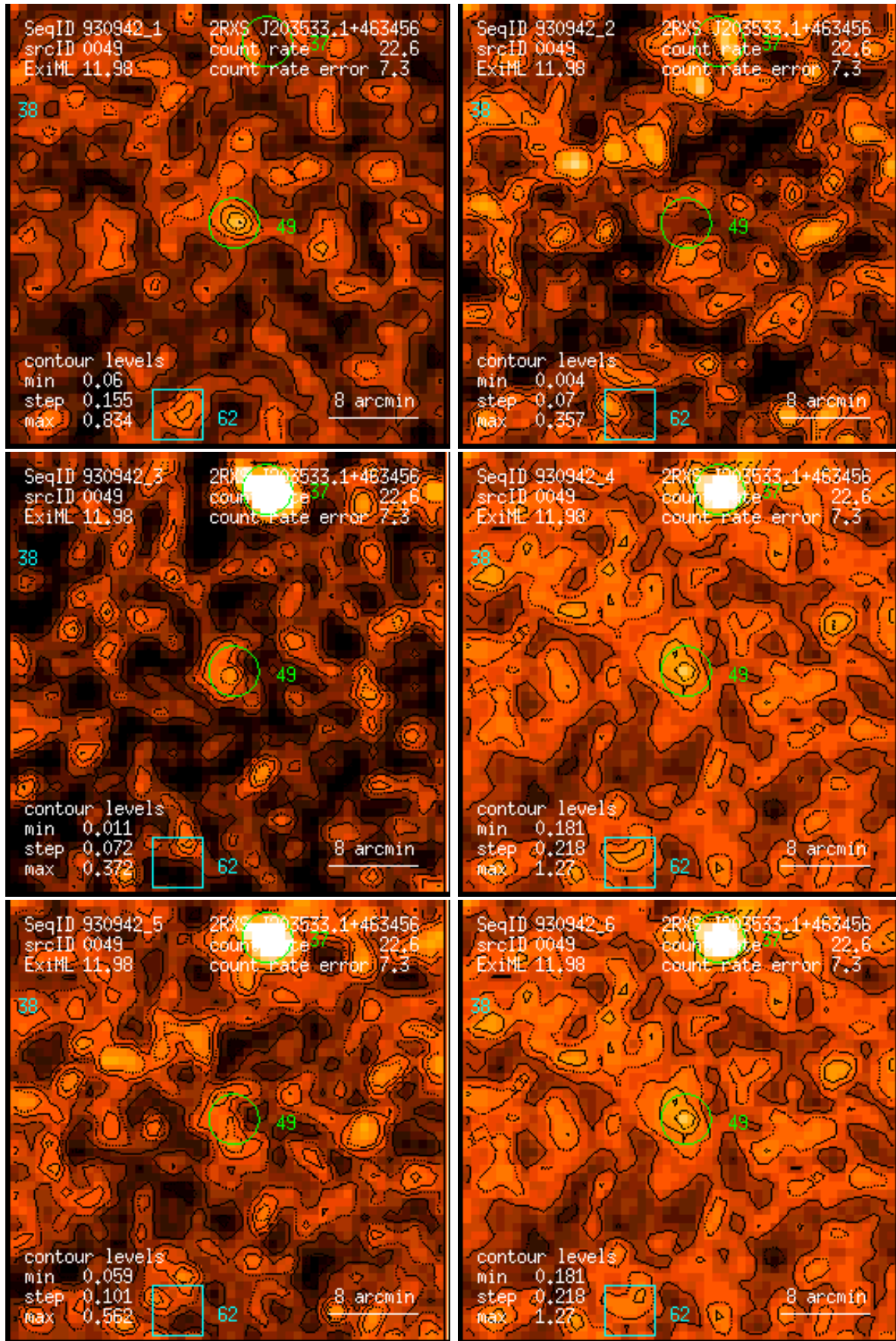
Figure 49: RASS 930942: detection 0049: band rate images, Gaussian filter: (1) PSPC channels 11 – 41, (2) 52 – 90, (3) 91 – 201, (4) 11 – 235, (5) 52 – 201, (6) 11 – 201. Broad band rates in counts/ks. Band rate contour levels in counts/ks/arcmin 2 .
