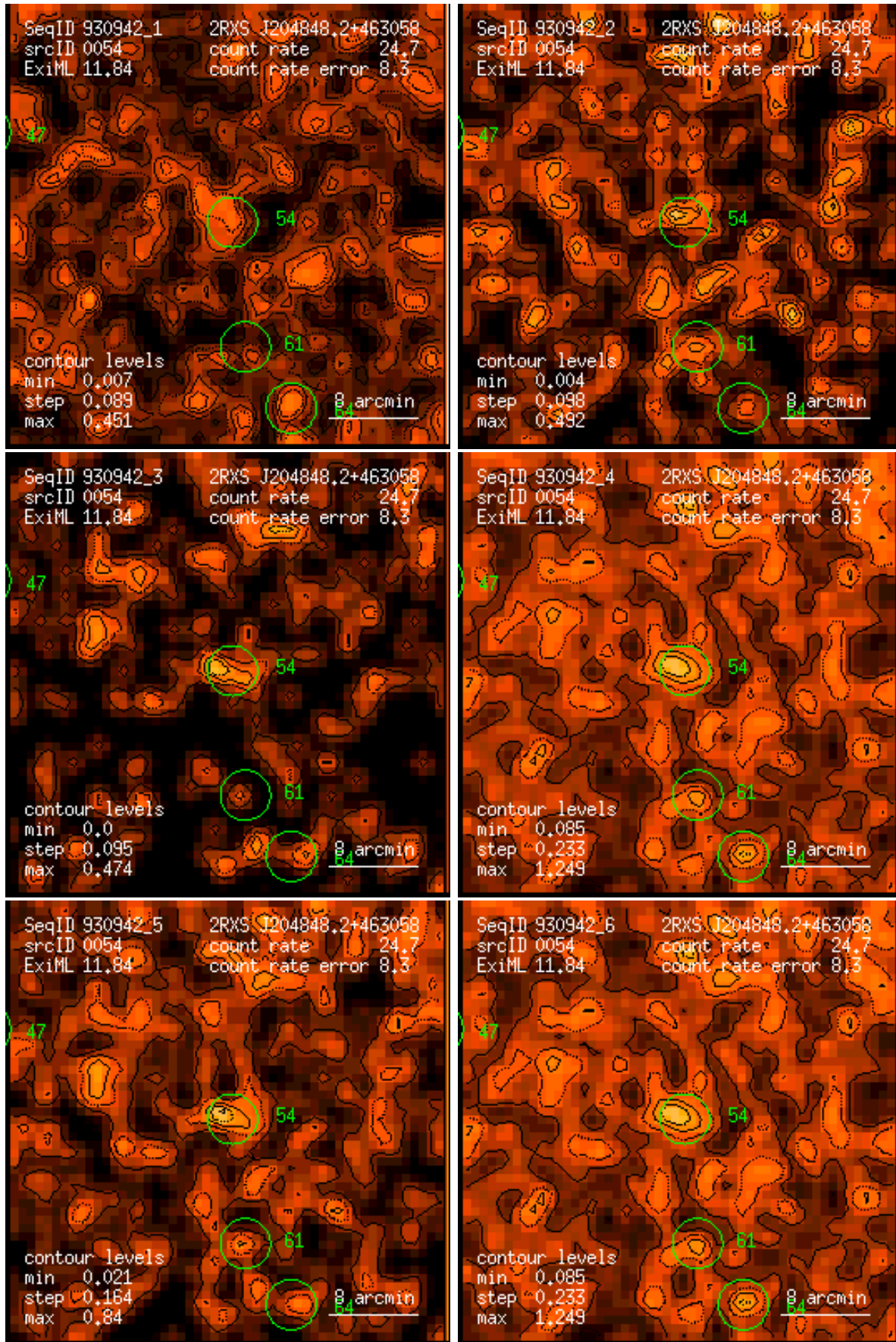
Figure 54: RASS 930942: detection 0054: band rate images, Gaussian filter: (1) PSPC channels 11 – 41, (2) 52 – 90, (3) 91 – 201, (4) 11 – 235, (5) 52 – 201, (6) 11 – 201. Broad band rates in counts/ks. Band rate contour levels in counts/ks/arcmin 2 .
