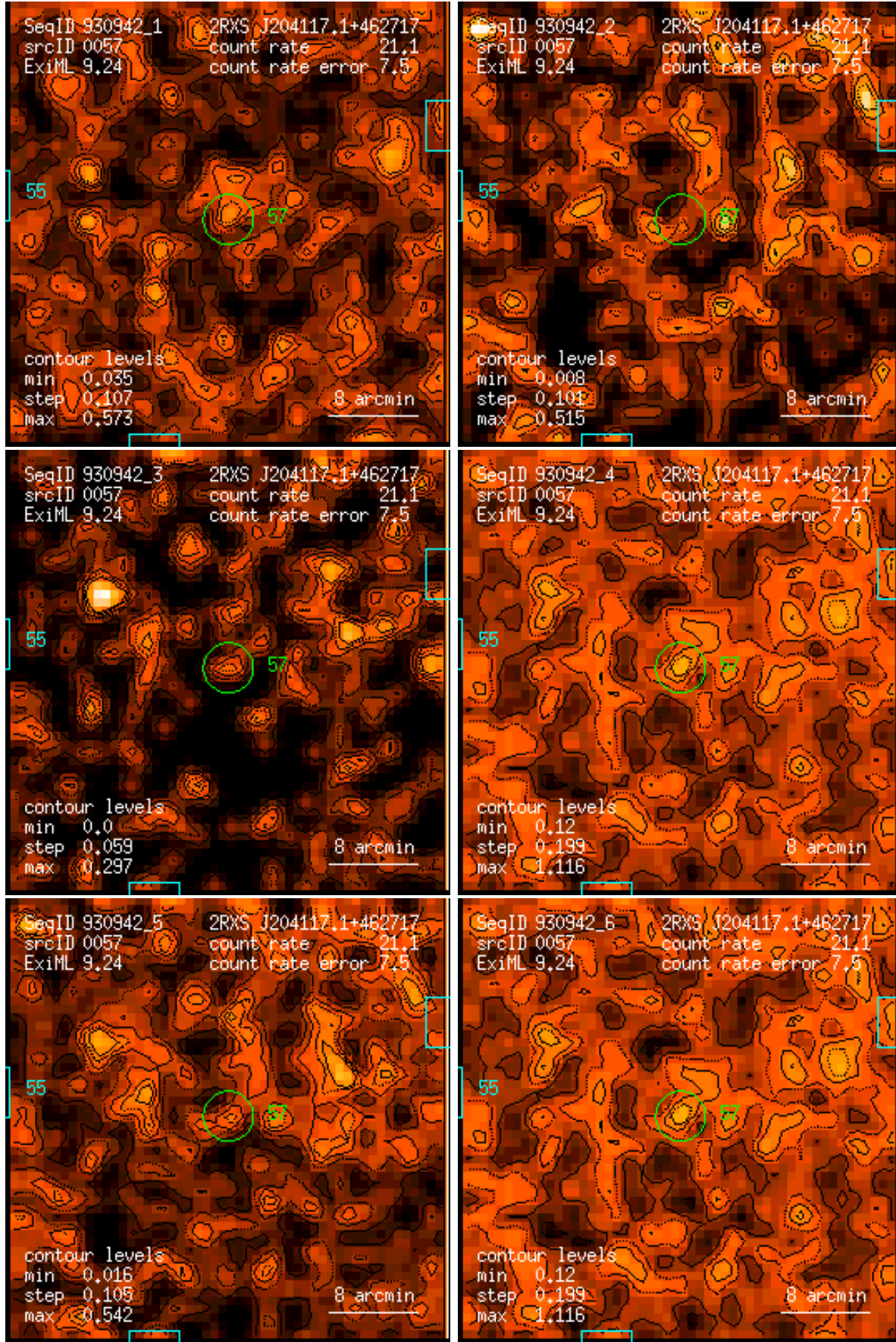
Figure 57: RASS 930942: detection 0057: band rate images, Gaussian filter: (1) PSPC channels 11 – 41, (2) 52 – 90, (3) 91 – 201, (4) 11 – 235, (5) 52 – 201, (6) 11 – 201. Broad band rates in counts/ks. Band rate contour levels in counts/ks/arcmin 2 .
