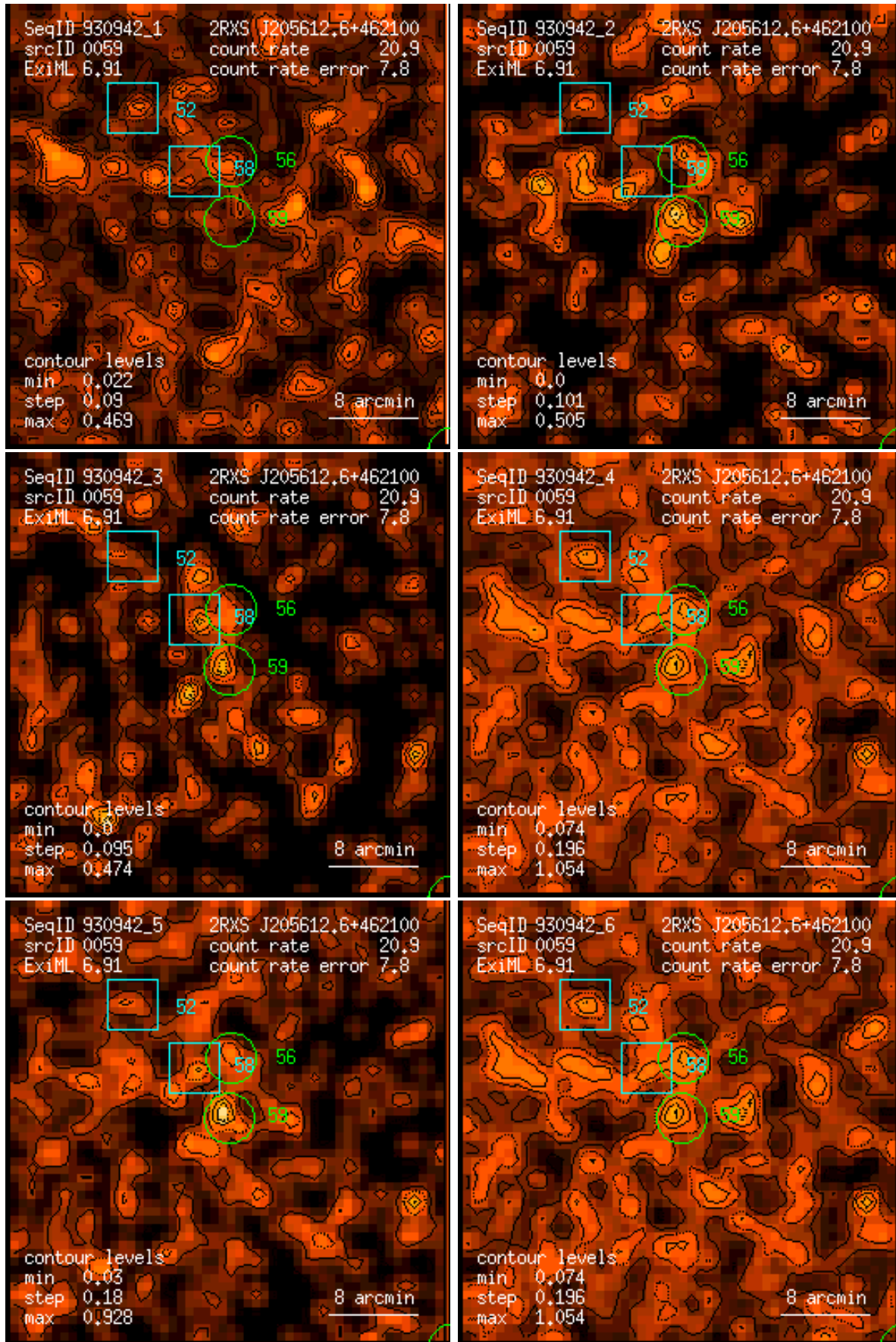
Figure 59: RASS 930942: detection 0059: band rate images, Gaussian filter: (1) PSPC channels 11 – 41, (2) 52 – 90, (3) 91 – 201, (4) 11 – 235, (5) 52 – 201, (6) 11 – 201. Broad band rates in counts/ks. Band rate contour levels in counts/ks/arcmin 2 .
