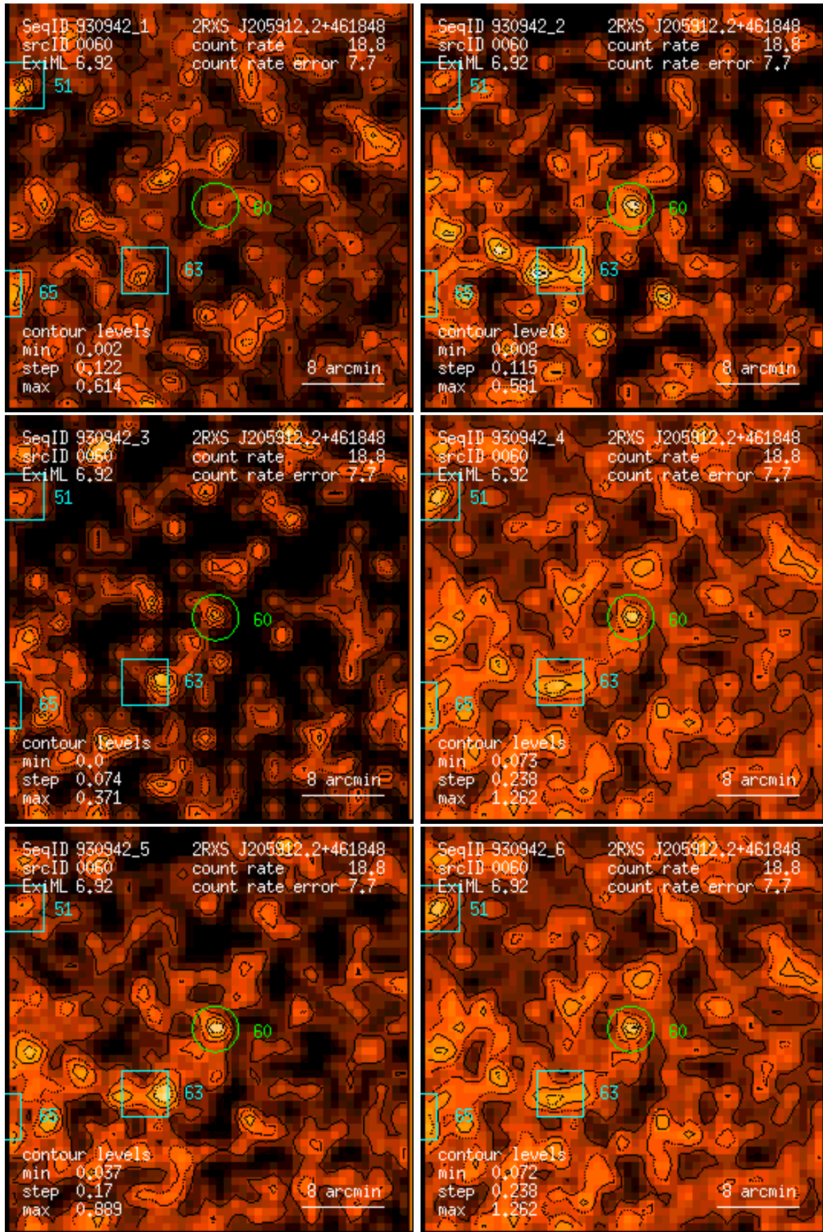
Figure 60: RASS 930942: detection 0060: band rate images, Gaussian filter: (1) PSPC channels 11 – 41, (2) 52 – 90, (3) 91 – 201, (4) 11 – 235, (5) 52 – 201, (6) 11 – 201. Broad band rates in counts/ks. Band rate contour levels in counts/ks/arcmin 2 .
