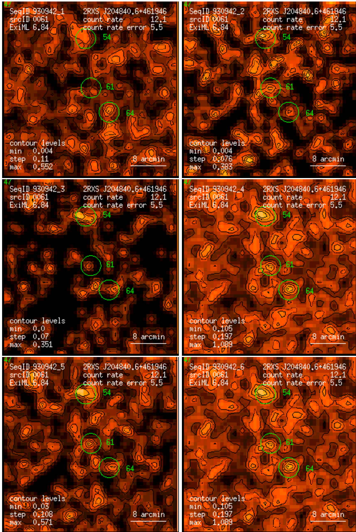
Figure 61: RASS 930942: detection 0061: band rate images, Gaussian filter: (1) PSPC channels 11 – 41, (2) 52 – 90, (3) 91 – 201, (4) 11 – 235, (5) 52 – 201, (6) 11 – 201. Broad band rates in counts/ks. Band rate contour levels in counts/ks/arcmin 2 .
