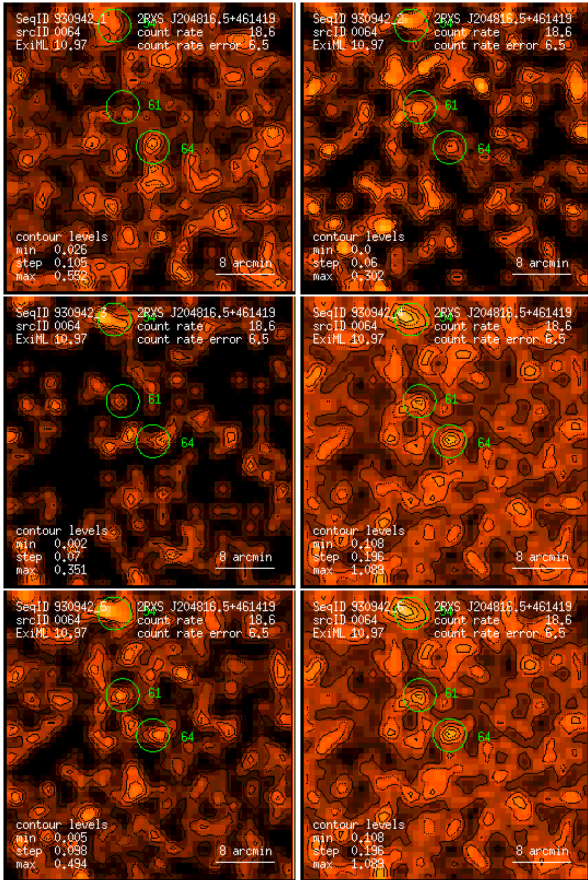
Figure 64: RASS 930942: detection 0064: band rate images, Gaussian filter: (1) PSPC channels 11 – 41, (2) 52 – 90, (3) 91 – 201, (4) 11 – 235, (5) 52 – 201, (6) 11 – 201. Broad band rates in counts/ks. Band rate contour levels in counts/ks/arcmin 2 .
